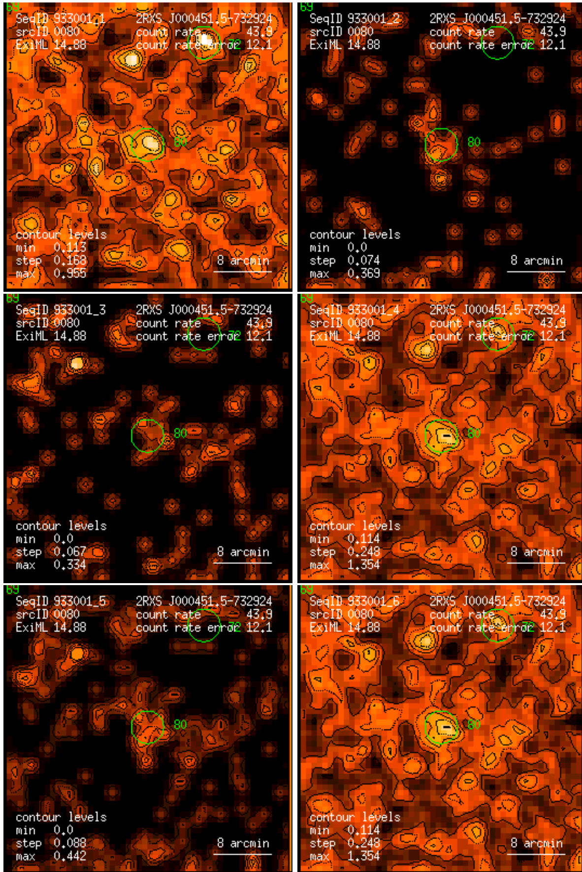
Figure 80: RASS 933001: detection 0080: band rate images, Gaussian filter: (1) PSPC channels 11 – 41, (2) 52 – 90, (3) 91 – 201, (4) 11 – 235, (5) 52 – 201, (6) 11 – 201. Broad band rates in counts/ks. Band rate contour levels in counts/ks/arcmin 2 .
