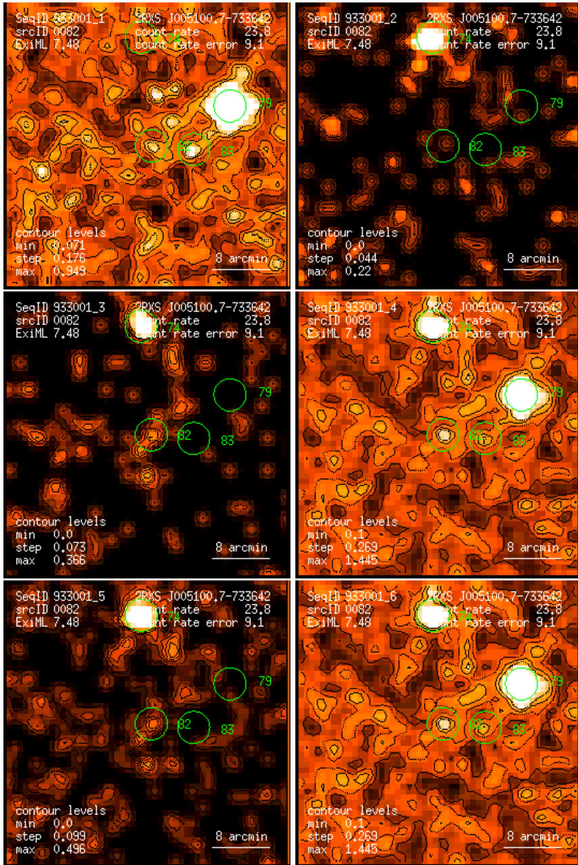
Figure 82: RASS 933001: detection 0082: band rate images, Gaussian filter: (1) PSPC channels 11 – 41, (2) 52 – 90, (3) 91 – 201, (4) 11 – 235, (5) 52 – 201, (6) 11 – 201. Broad band rates in counts/ks. Band rate contour levels in counts/ks/arcmin 2 .
