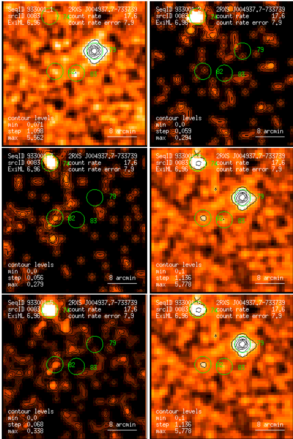
Figure 83: RASS 933001: detection 0083: band rate images, Gaussian filter: (1) PSPC channels 11 – 41, (2) 52 – 90, (3) 91 – 201, (4) 11 – 235, (5) 52 – 201, (6) 11 – 201. Broad band rates in counts/ks. Band rate contour levels in counts/ks/arcmin 2 .
