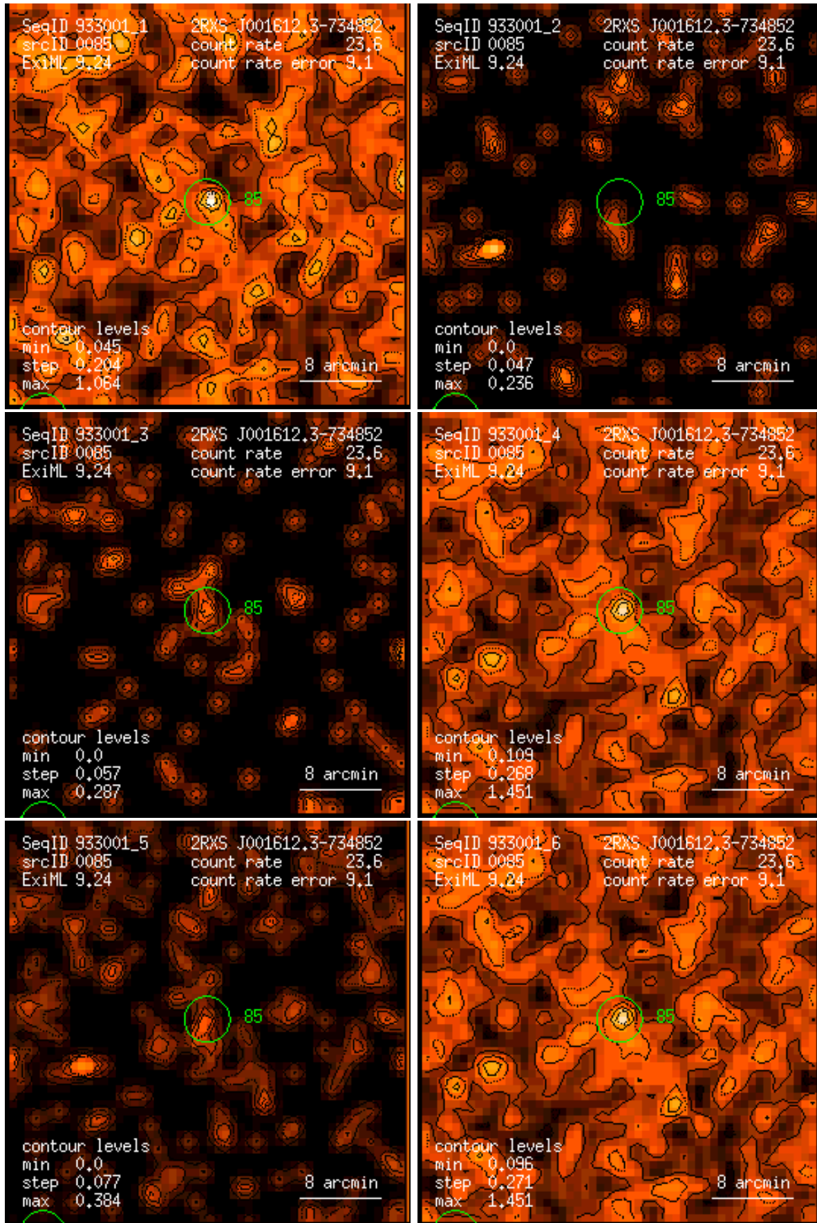
Figure 85: RASS 933001: detection 0085: band rate images, Gaussian filter: (1) PSPC channels 11 – 41, (2) 52 – 90, (3) 91 – 201, (4) 11 – 235, (5) 52 – 201, (6) 11 – 201. Broad band rates in counts/ks. Band rate contour levels in counts/ks/arcmin 2 .
