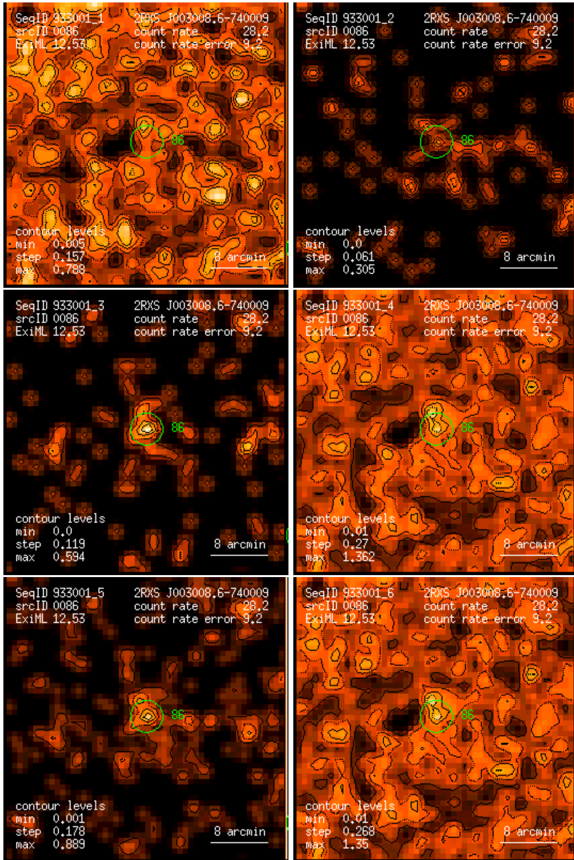
Figure 86: RASS 933001: detection 0086: band rate images, Gaussian filter: (1) PSPC channels 11 – 41, (2) 52 – 90, (3) 91 – 201, (4) 11 – 235, (5) 52 – 201, (6) 11 – 201. Broad band rates in counts/ks. Band rate contour levels in counts/ks/arcmin 2 .
