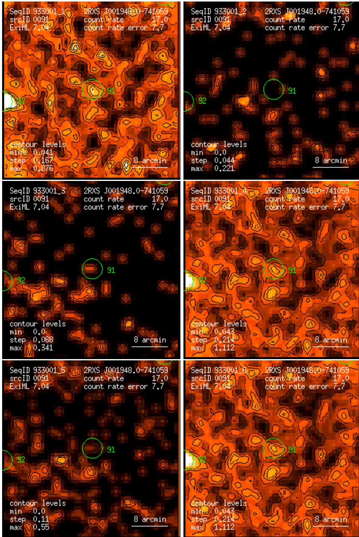
Figure 91: RASS 933001: detection 0091: band rate images, Gaussian filter: (1) PSPC channels 11 – 41, (2) 52 – 90, (3) 91 – 201, (4) 11 – 235, (5) 52 – 201, (6) 11 – 201. Broad band rates in counts/ks. Band rate contour levels in counts/ks/arcmin 2 .
