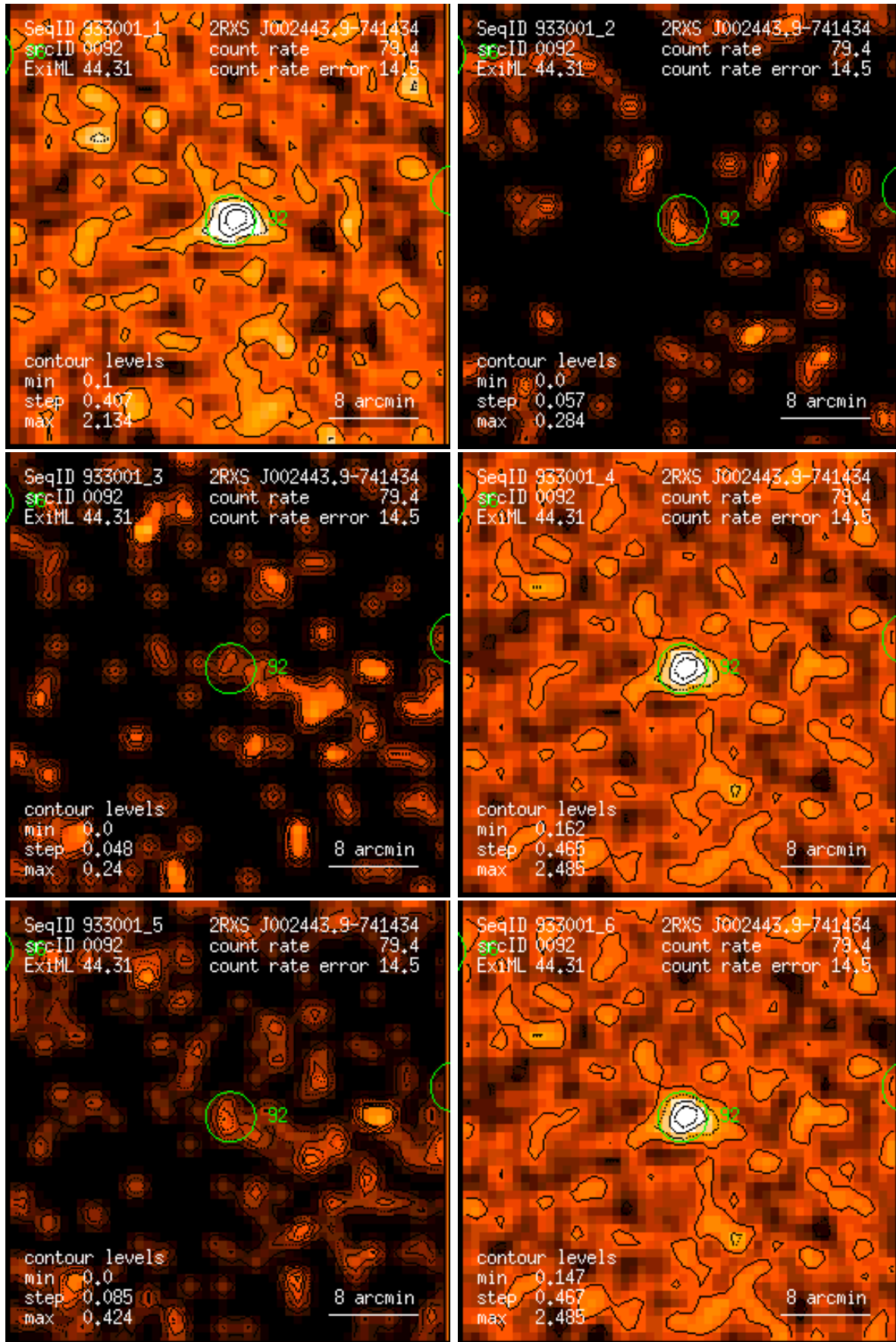
Figure 92: RASS 933001: detection 0092: band rate images, Gaussian filter: (1) PSPC channels 11 – 41, (2) 52 – 90, (3) 91 – 201, (4) 11 – 235, (5) 52 – 201, (6) 11 – 201. Broad band rates in counts/ks. Band rate contour levels in counts/ks/arcmin 2 .
