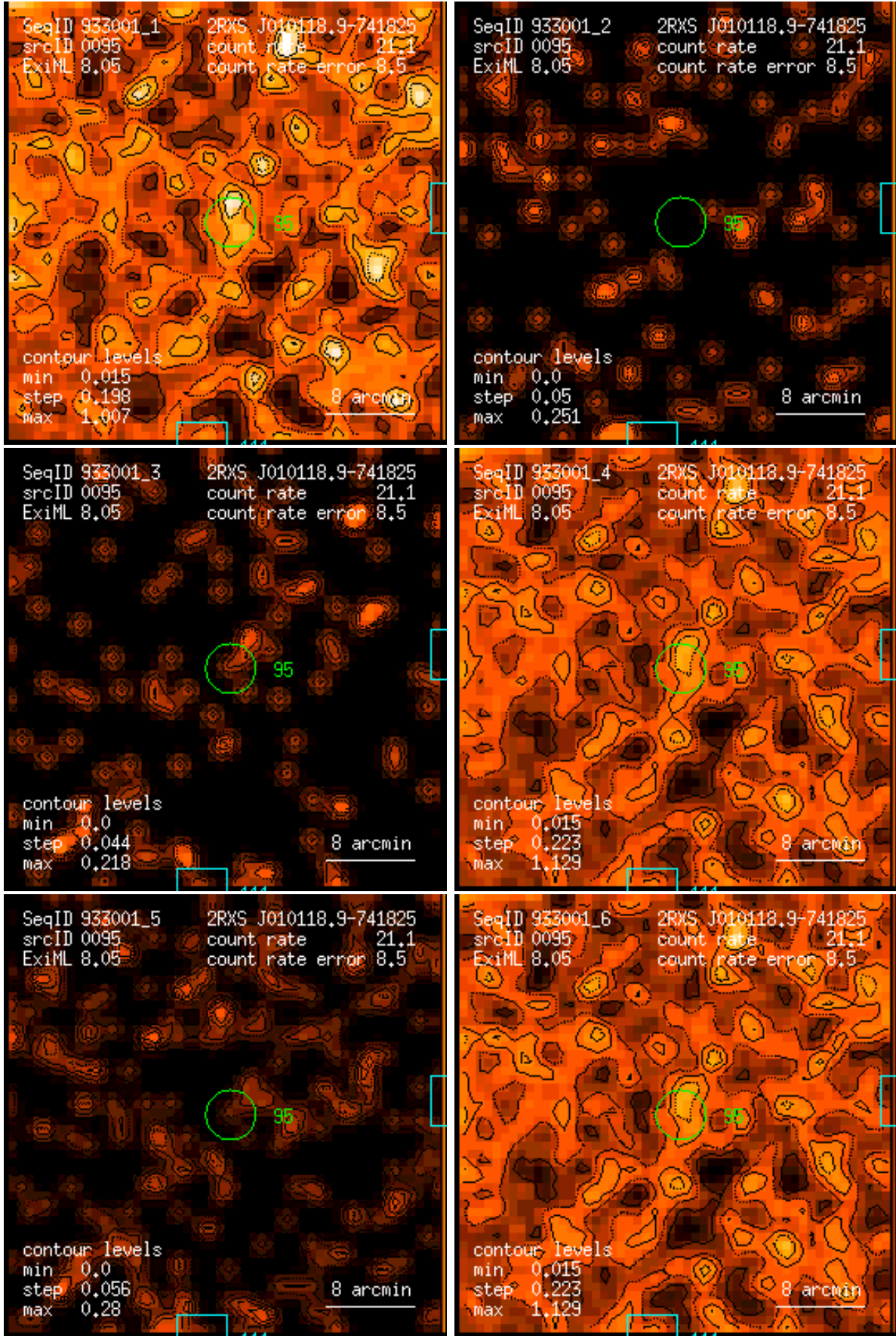
Figure 95: RASS 933001: detection 0095: band rate images, Gaussian filter: (1) PSPC channels 11 – 41, (2) 52 – 90, (3) 91 – 201, (4) 11 – 235, (5) 52 – 201, (6) 11 – 201. Broad band rates in counts/ks. Band rate contour levels in counts/ks/arcmin 2 .
