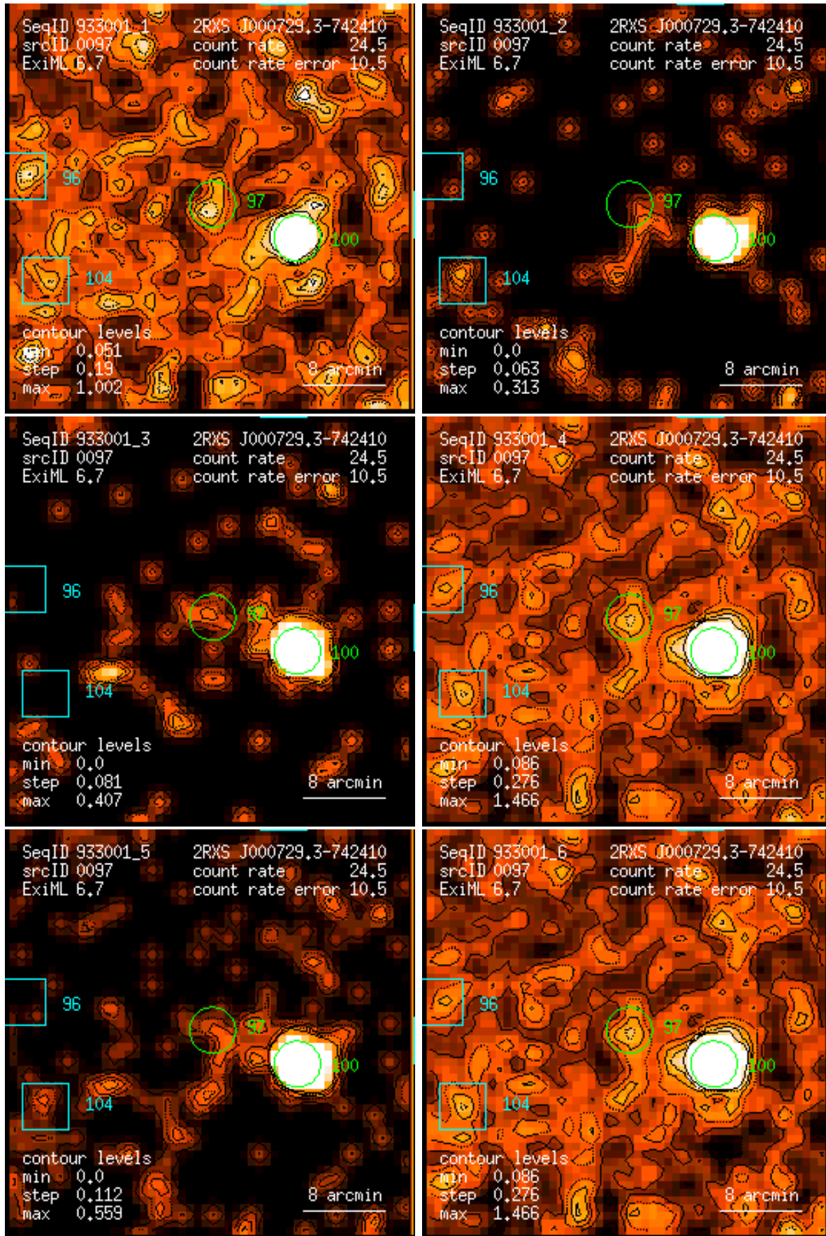
Figure 97: RASS 933001: detection 0097: band rate images, Gaussian filter: (1) PSPC channels 11 – 41, (2) 52 – 90, (3) 91 – 201, (4) 11 – 235, (5) 52 – 201, (6) 11 – 201. Broad band rates in counts/ks. Band rate contour levels in counts/ks/arcmin 2 .
