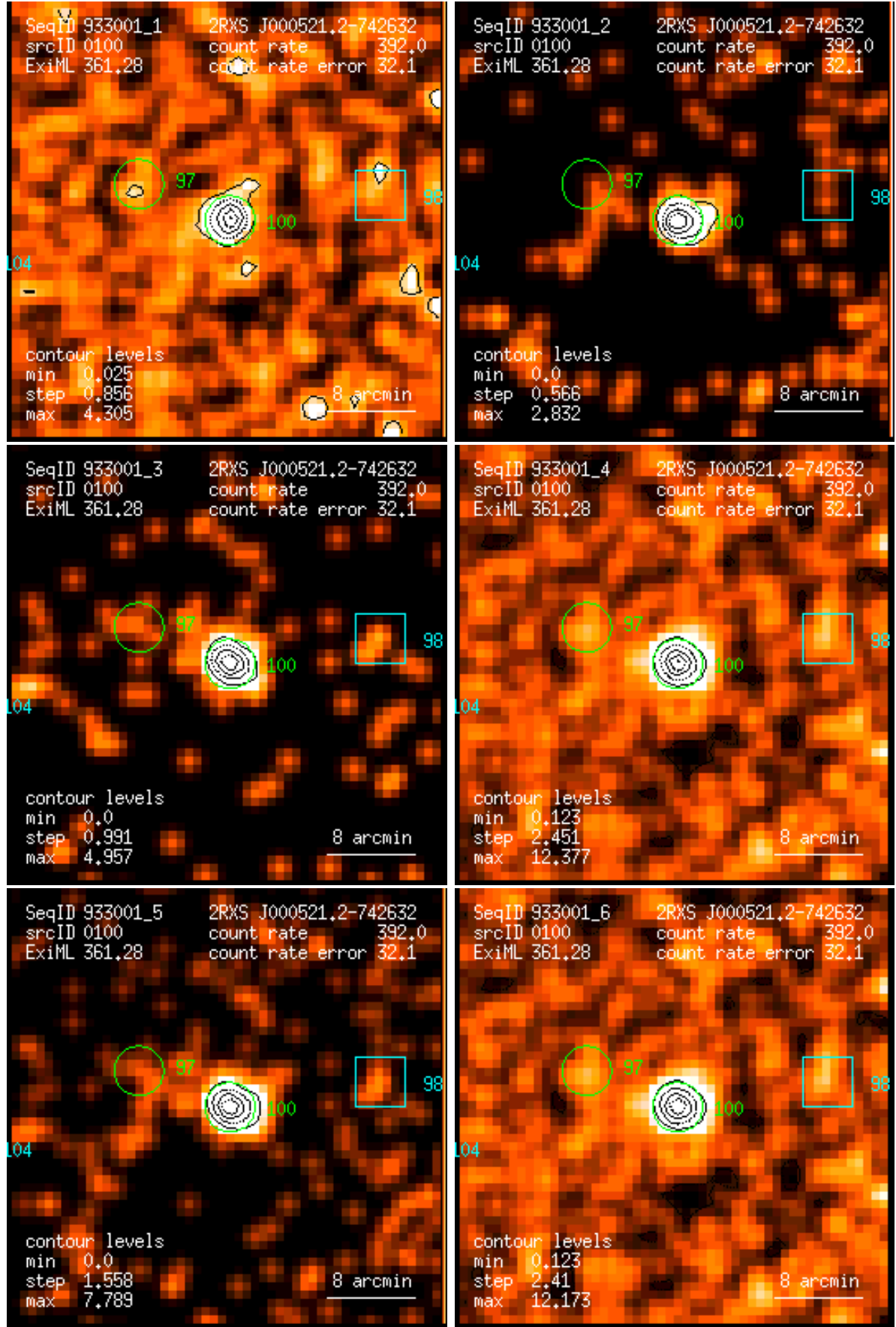
Figure 100: RASS 933001: detection 0100: band rate images, Gaussian filter: (1) PSPC channels 11 – 41, (2) 52 – 90, (3) 91 – 201, (4) 11 – 235, (5) 52 – 201, (6) 11 – 201. Broad band rates in counts/ks. Band rate contour levels in counts/ks/arcmin 2 .
