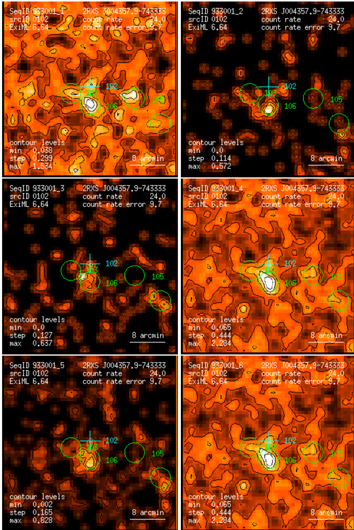
Figure 102: RASS 933001: detection 0102: band rate images, Gaussian filter: (1) PSPC channels 11 – 41, (2) 52 – 90, (3) 91 – 201, (4) 11 – 235, (5) 52 – 201, (6) 11 – 201. Broad band rates in counts/ks. Band rate contour levels in counts/ks/arcmin 2 .
