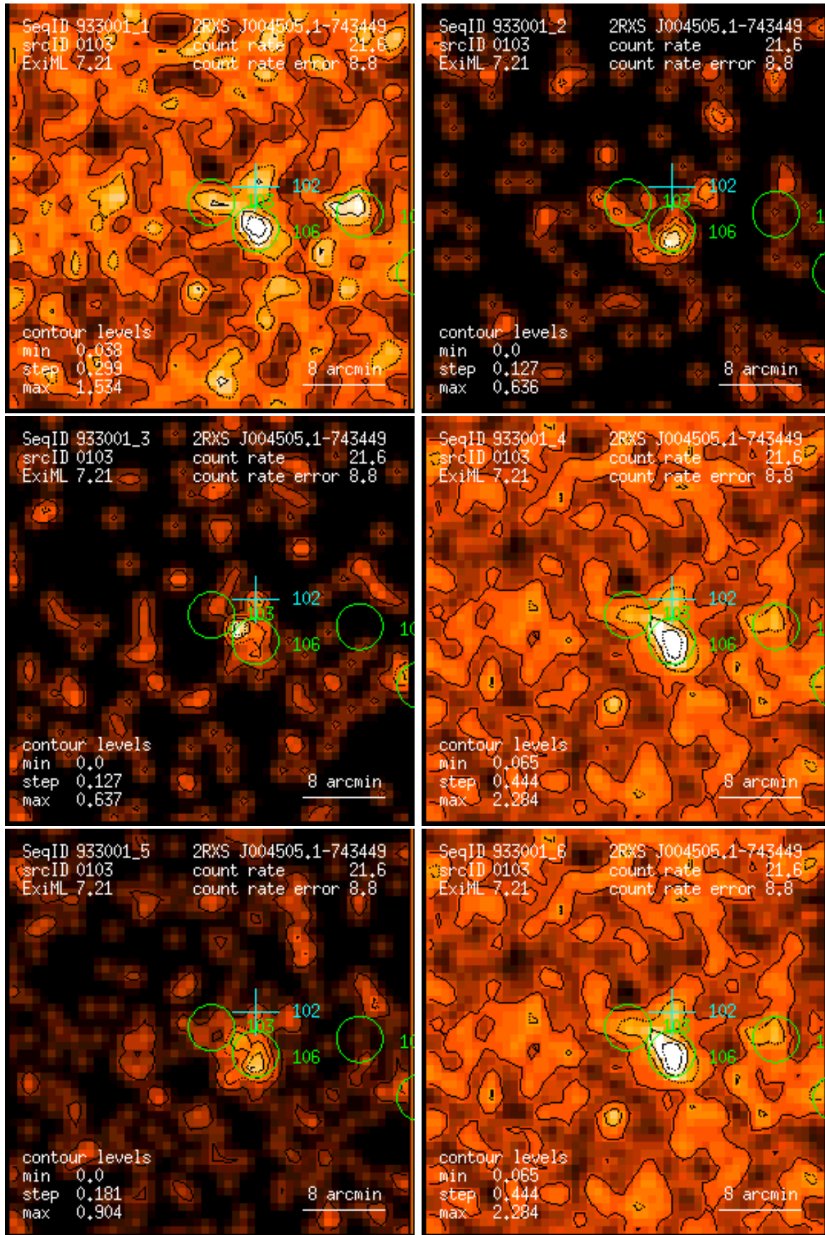
Figure 103: RASS 933001: detection 0103: band rate images, Gaussian filter: (1) PSPC channels 11 – 41, (2) 52 – 90, (3) 91 – 201, (4) 11 – 235, (5) 52 – 201, (6) 11 – 201. Broad band rates in counts/ks. Band rate contour levels in counts/ks/arcmin 2 .
