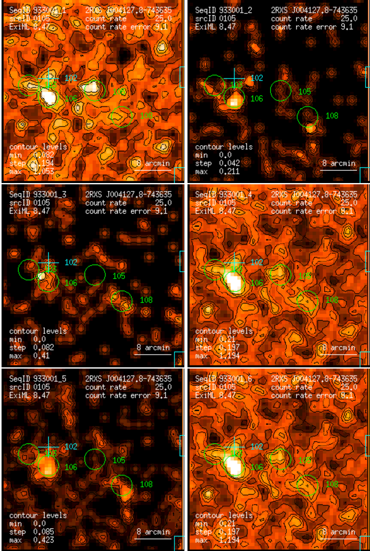
Figure 105: RASS 933001: detection 0105: band rate images, Gaussian filter: (1) PSPC channels 11 – 41, (2) 52 – 90, (3) 91 – 201, (4) 11 – 235, (5) 52 – 201, (6) 11 – 201. Broad band rates in counts/ks. Band rate contour levels in counts/ks/arcmin 2 .
