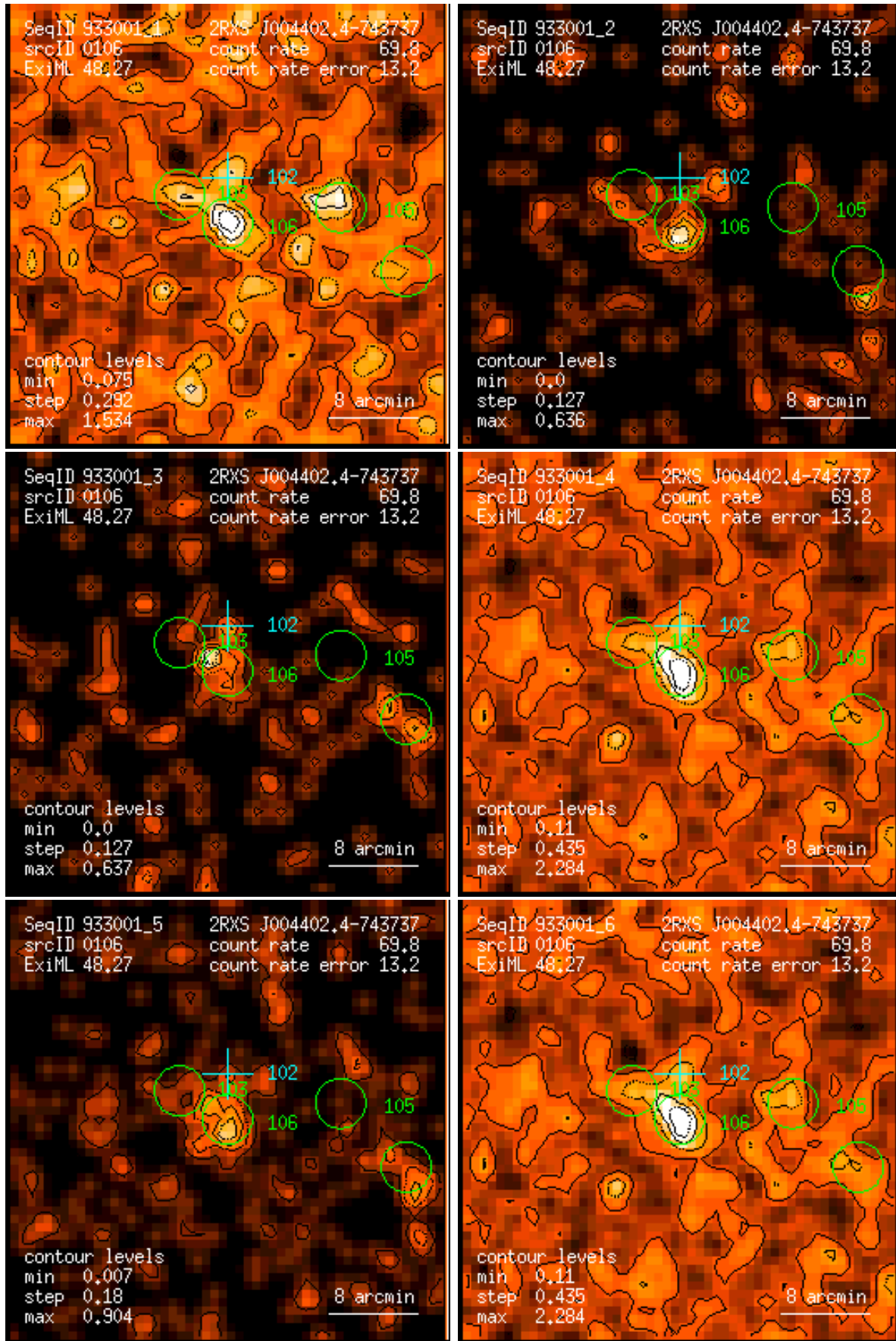
Figure 106: RASS 933001: detection 0106: band rate images, Gaussian filter: (1) PSPC channels 11 – 41, (2) 52 – 90, (3) 91 – 201, (4) 11 – 235, (5) 52 – 201, (6) 11 – 201. Broad band rates in counts/ks. Band rate contour levels in counts/ks/arcmin 2 .
