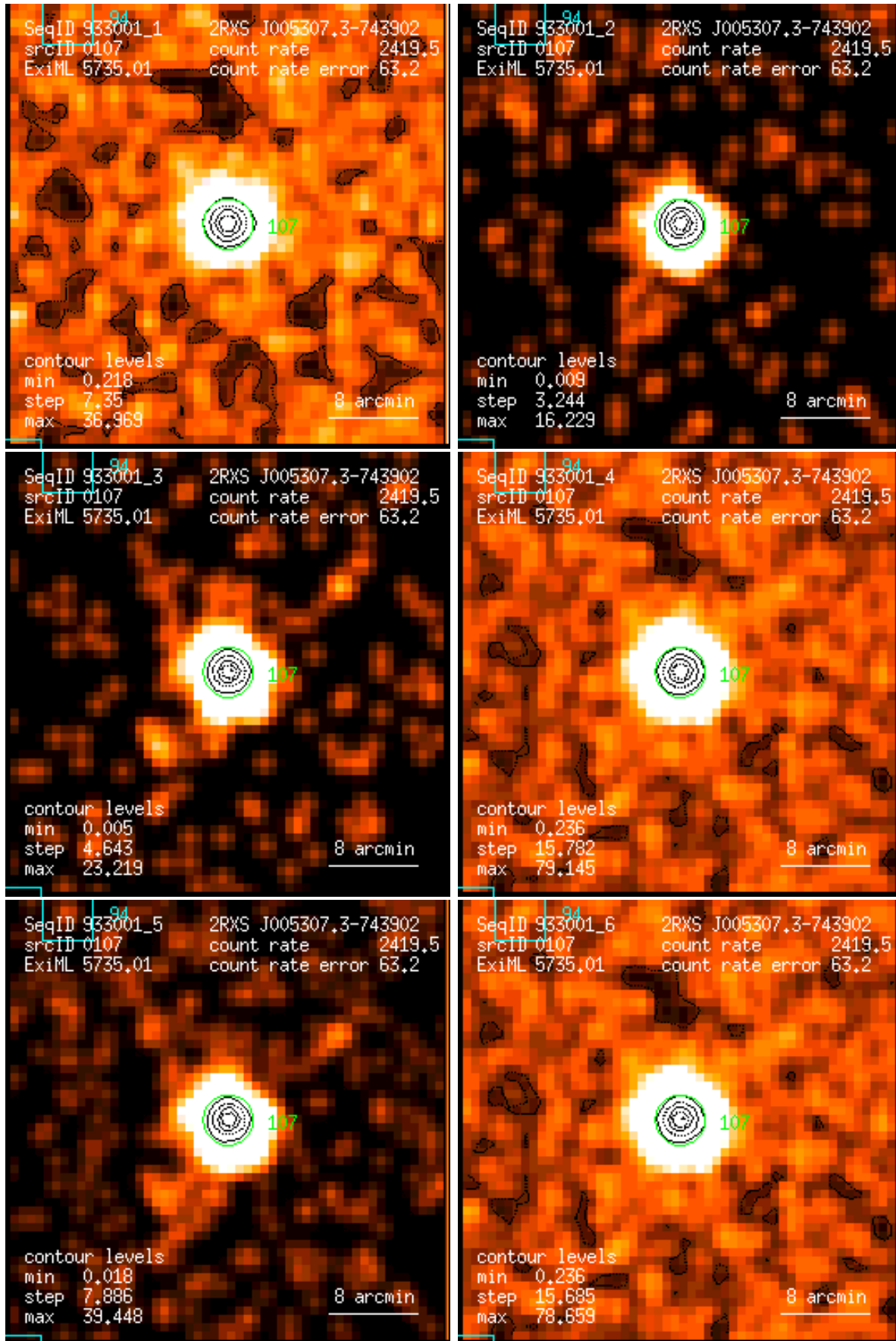
Figure 107: RASS 933001: detection 0107: band rate images, Gaussian filter: (1) PSPC channels 11 – 41, (2) 52 – 90, (3) 91 – 201, (4) 11 – 235, (5) 52 – 201, (6) 11 – 201. Broad band rates in counts/ks. Band rate contour levels in counts/ks/arcmin 2 .
