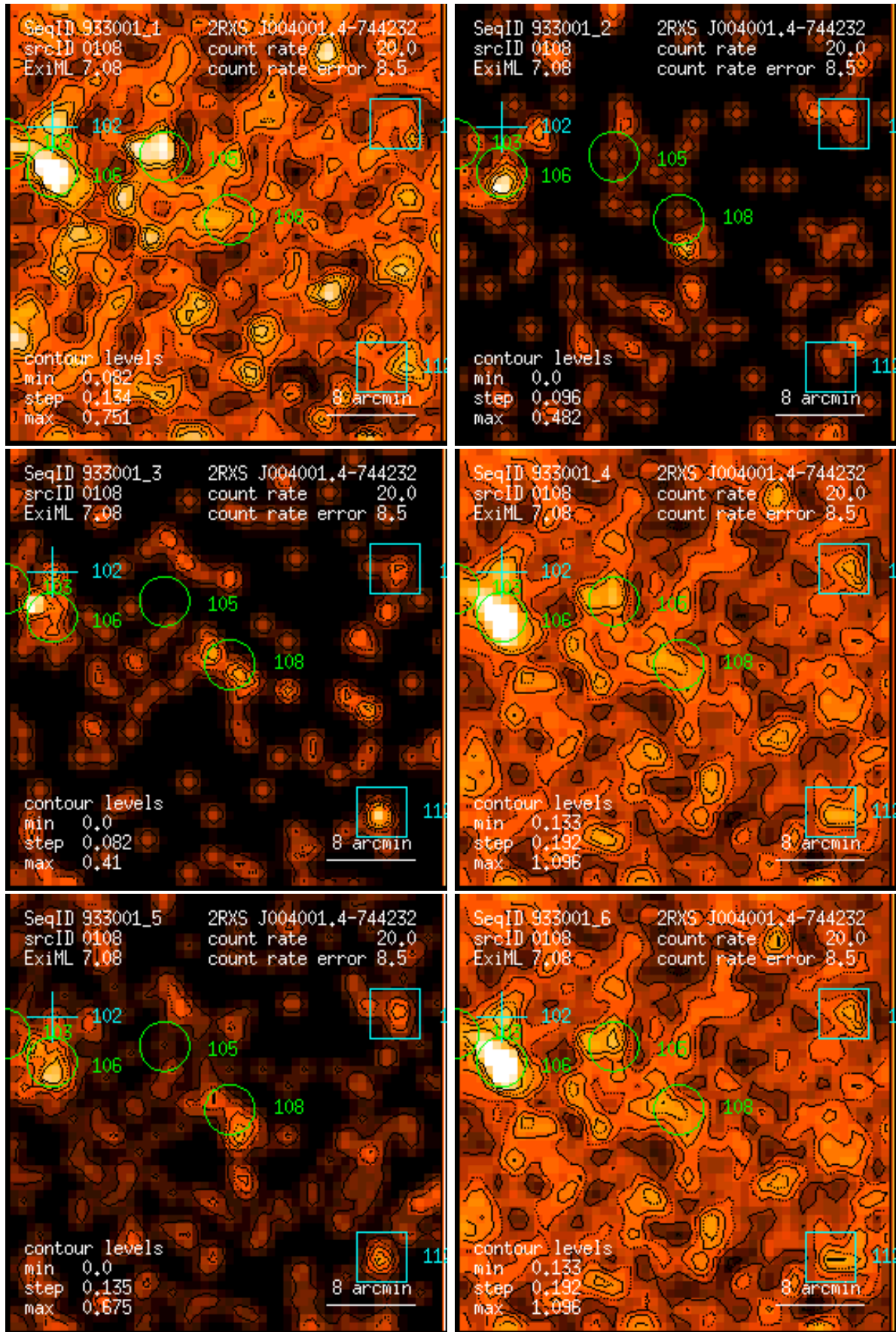
Figure 108: RASS 933001: detection 0108: band rate images, Gaussian filter: (1) PSPC channels 11 – 41, (2) 52 – 90, (3) 91 – 201, (4) 11 – 235, (5) 52 – 201, (6) 11 – 201. Broad band rates in counts/ks. Band rate contour levels in counts/ks/arcmin 2 .
