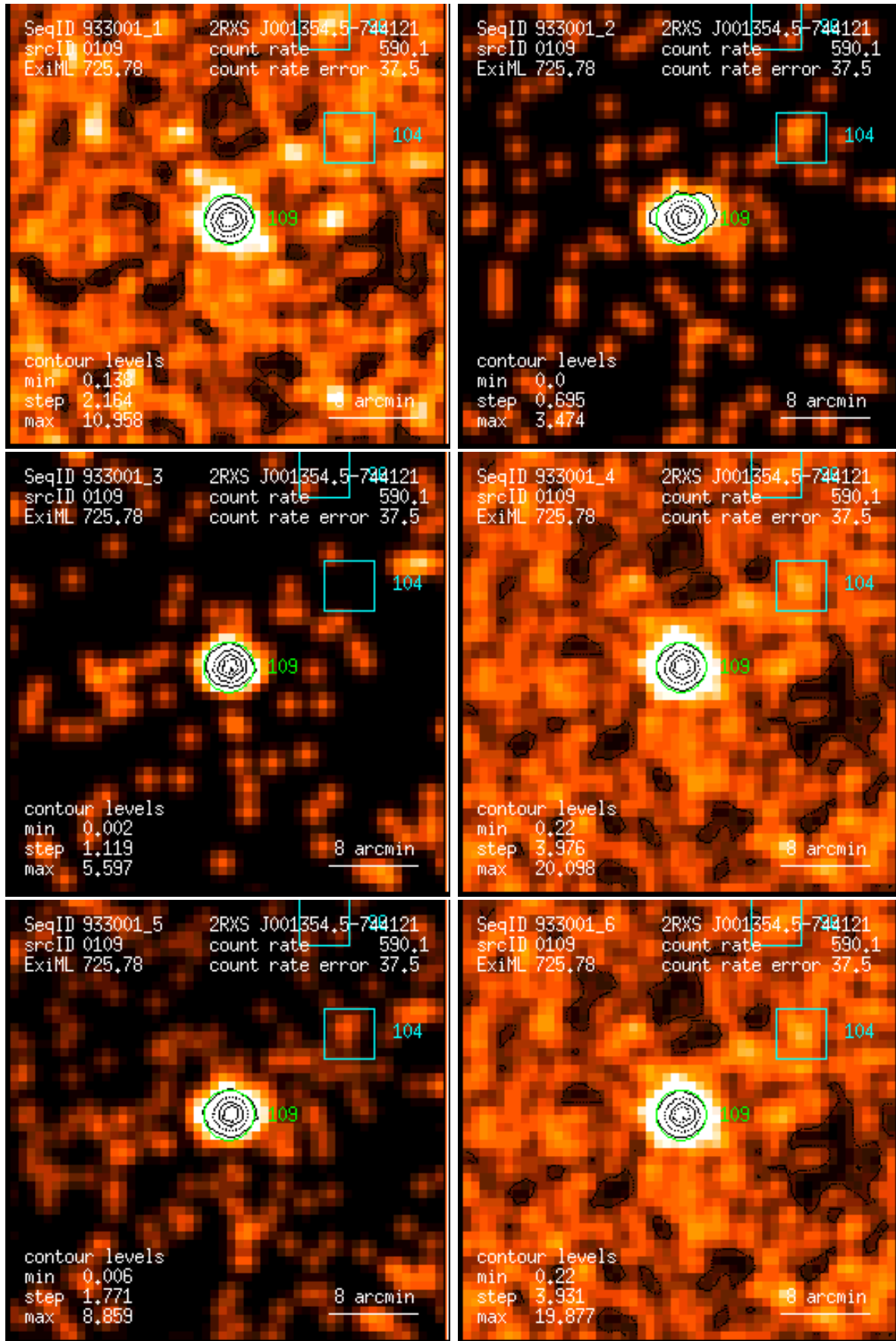
Figure 109: RASS 933001: detection 0109: band rate images, Gaussian filter: (1) PSPC channels 11 – 41, (2) 52 – 90, (3) 91 – 201, (4) 11 – 235, (5) 52 – 201, (6) 11 – 201. Broad band rates in counts/ks. Band rate contour levels in counts/ks/arcmin 2 .
