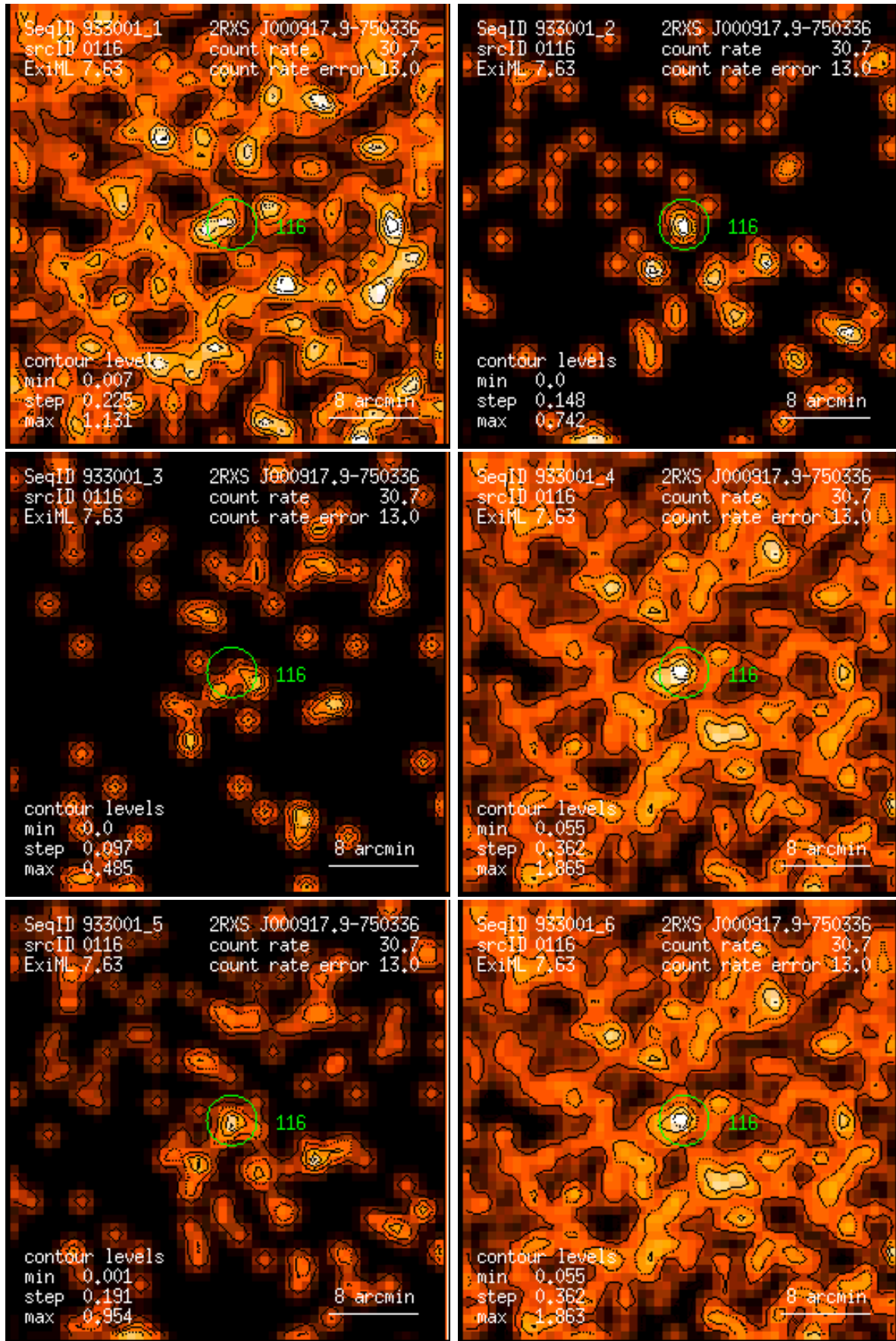
Figure 116: RASS 933001: detection 0116: band rate images, Gaussian filter: (1) PSPC channels 11 – 41, (2) 52 – 90, (3) 91 – 201, (4) 11 – 235, (5) 52 – 201, (6) 11 – 201. Broad band rates in counts/ks. Band rate contour levels in counts/ks/arcmin 2 .
