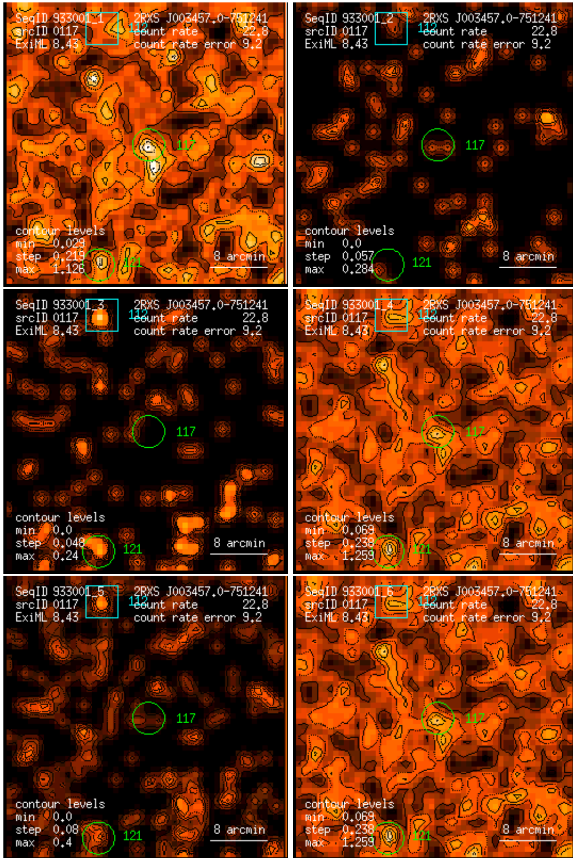
Figure 117: RASS 933001: detection 0117: band rate images, Gaussian filter: (1) PSPC channels 11 – 41, (2) 52 – 90, (3) 91 – 201, (4) 11 – 235, (5) 52 – 201, (6) 11 – 201. Broad band rates in counts/ks. Band rate contour levels in counts/ks/arcmin 2 .
