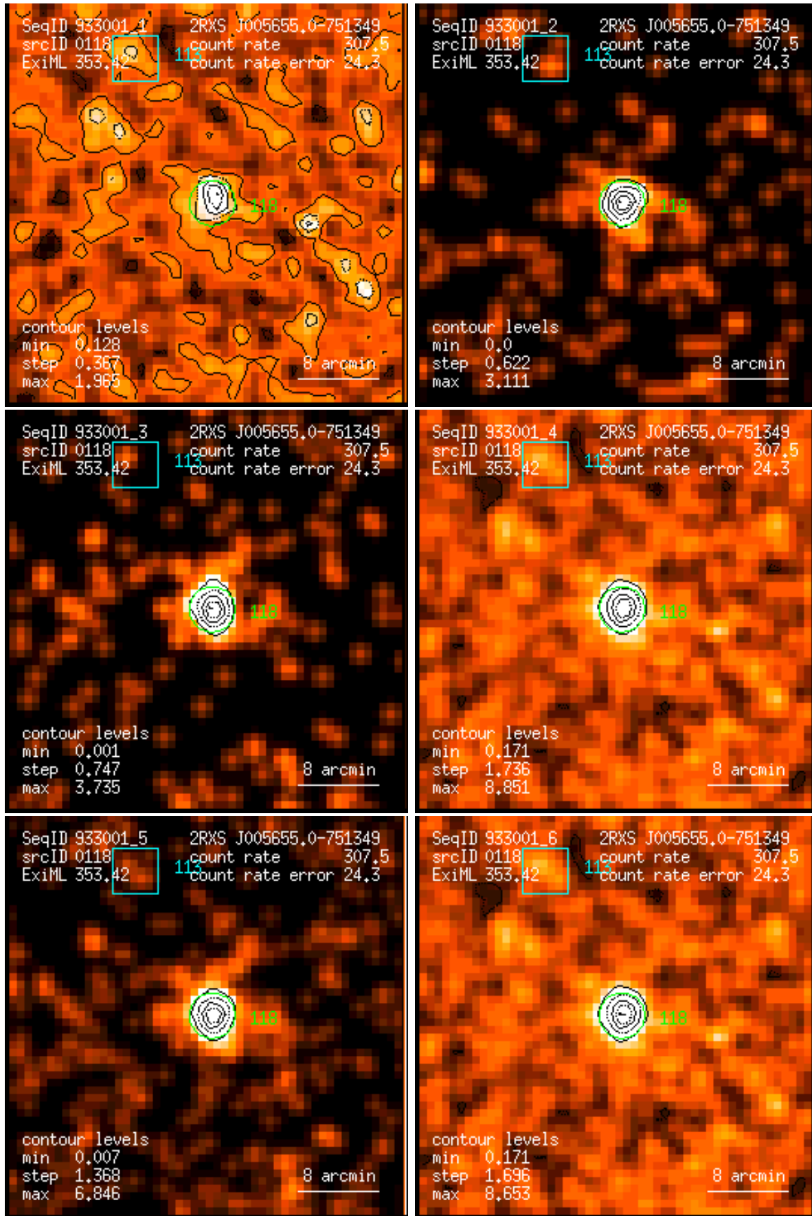
Figure 118: RASS 933001: detection 0118: band rate images, Gaussian filter: (1) PSPC channels 11 – 41, (2) 52 – 90, (3) 91 – 201, (4) 11 – 235, (5) 52 – 201, (6) 11 – 201. Broad band rates in counts/ks. Band rate contour levels in counts/ks/arcmin 2 .
