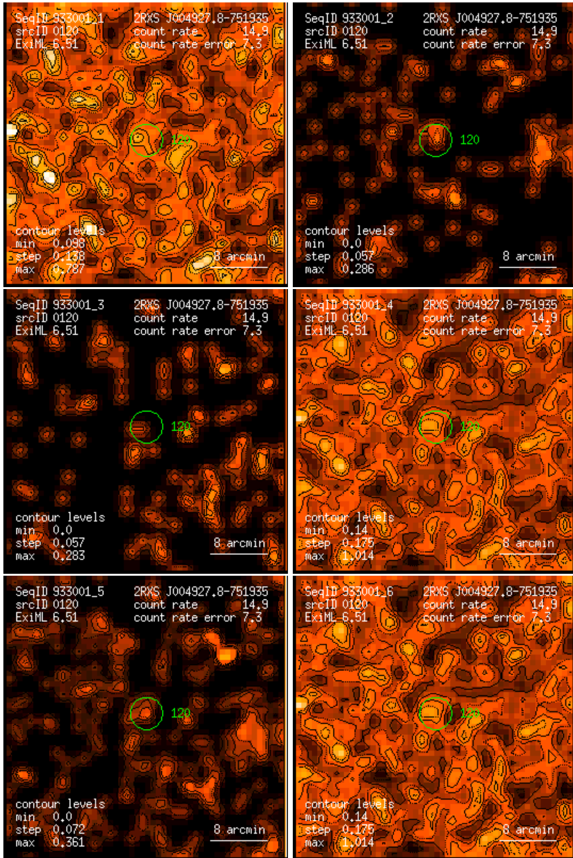
Figure 120: RASS 933001: detection 0120: band rate images, Gaussian filter: (1) PSPC channels 11 – 41, (2) 52 – 90, (3) 91 – 201, (4) 11 – 235, (5) 52 – 201, (6) 11 – 201. Broad band rates in counts/ks. Band rate contour levels in counts/ks/arcmin 2 .
