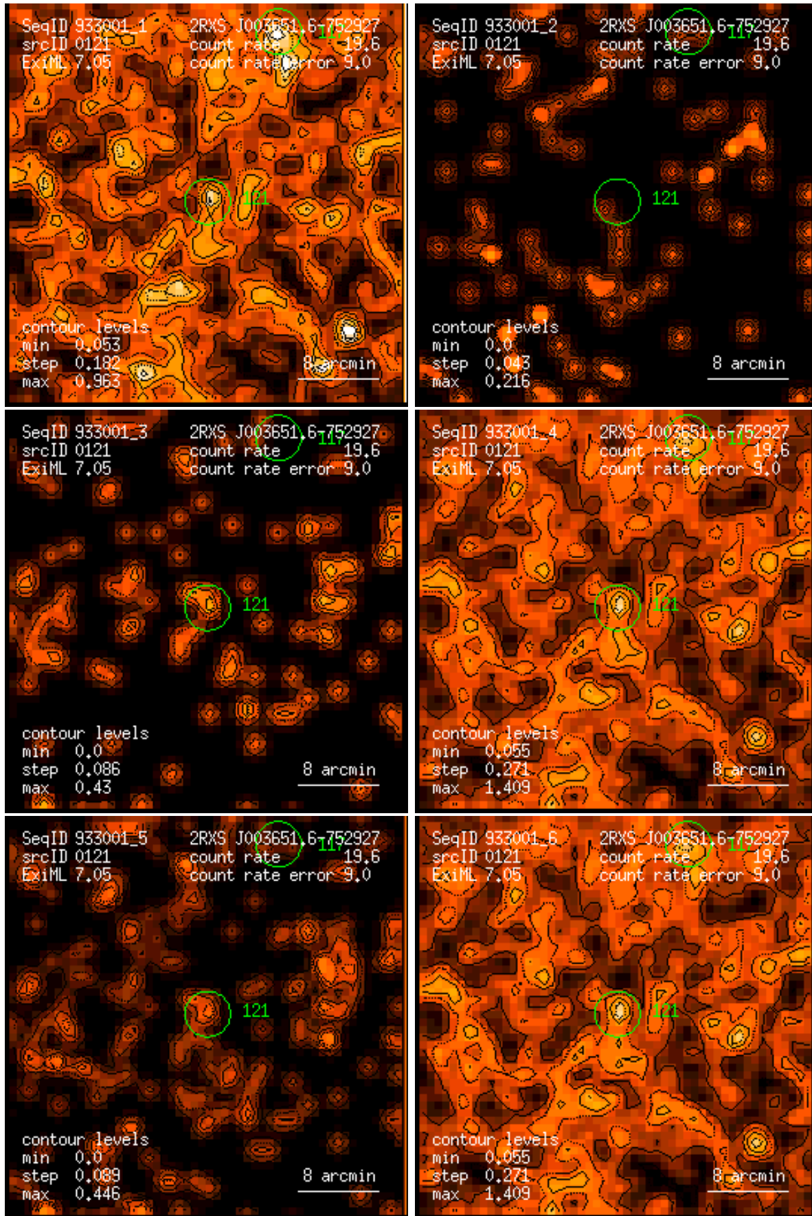
Figure 121: RASS 933001: detection 0121: band rate images, Gaussian filter: (1) PSPC channels 11 – 41, (2) 52 – 90, (3) 91 – 201, (4) 11 – 235, (5) 52 – 201, (6) 11 – 201. Broad band rates in counts/ks. Band rate contour levels in counts/ks/arcmin 2 .
