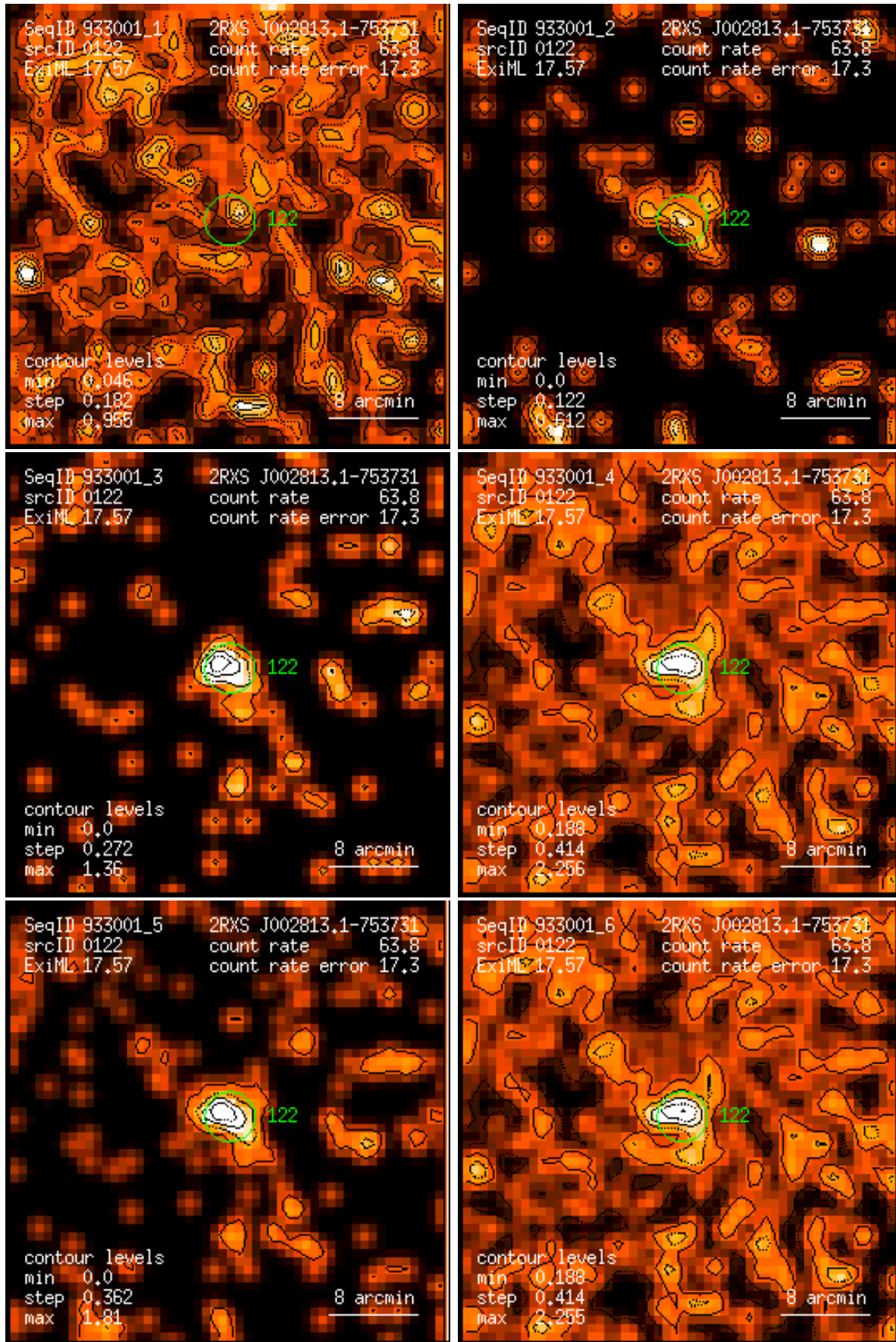
Figure 122: RASS 933001: detection 0122: band rate images, Gaussian filter: (1) PSPC channels 11 – 41, (2) 52 – 90, (3) 91 – 201, (4) 11 – 235, (5) 52 – 201, (6) 11 – 201. Broad band rates in counts/ks. Band rate contour levels in counts/ks/arcmin 2 .
