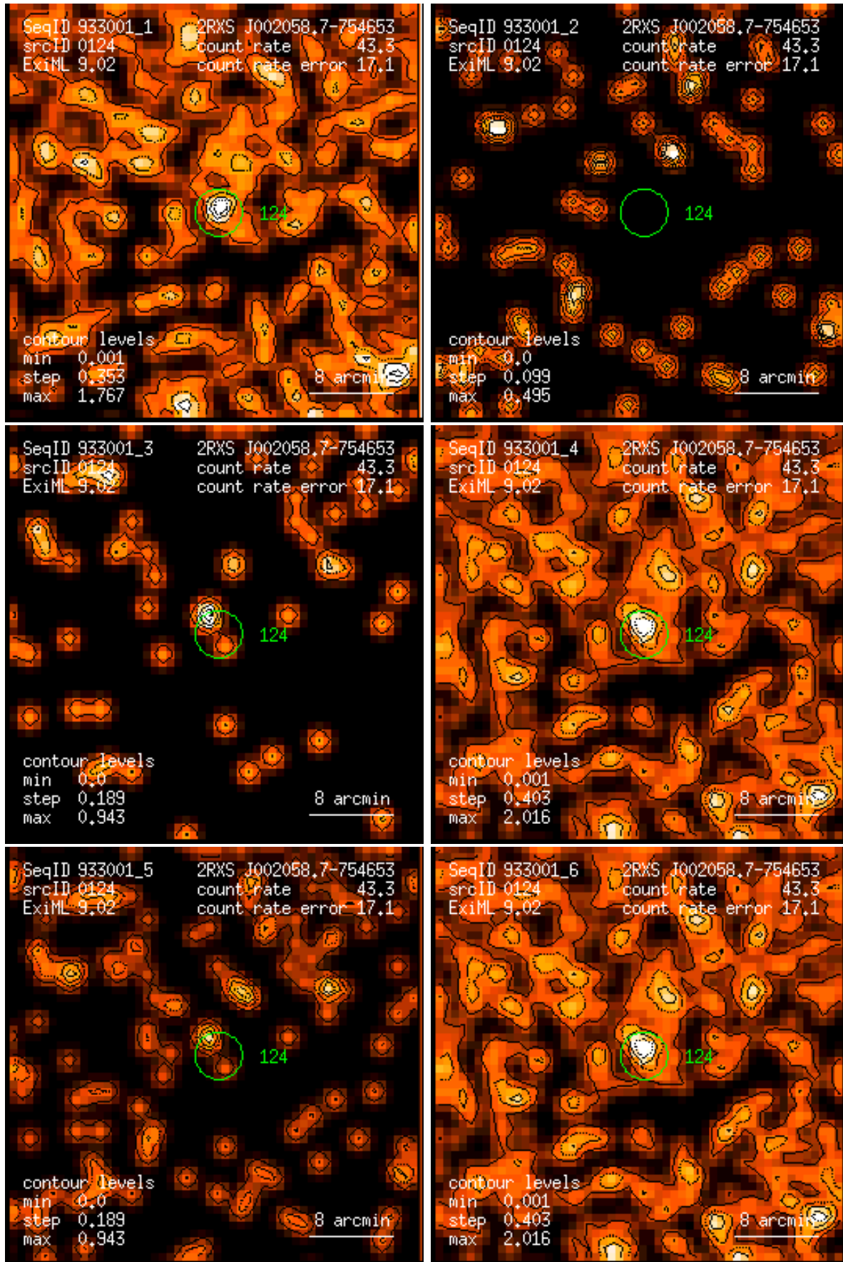
Figure 124: RASS 933001: detection 0124: band rate images, Gaussian filter: (1) PSPC channels 11 – 41, (2) 52 – 90, (3) 91 – 201, (4) 11 – 235, (5) 52 – 201, (6) 11 – 201. Broad band rates in counts/ks. Band rate contour levels in counts/ks/arcmin 2 .
