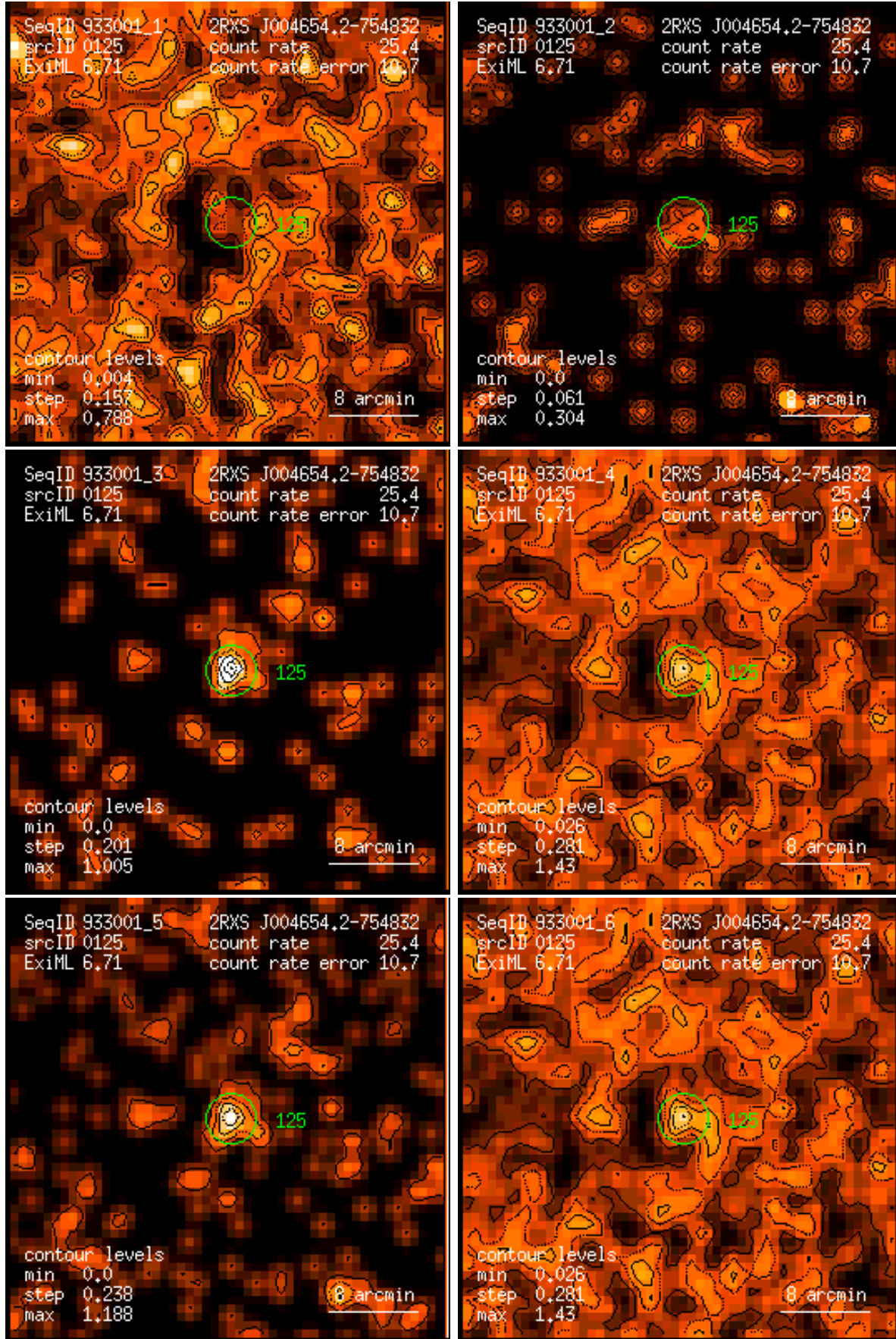
Figure 125: RASS 933001: detection 0125: band rate images, Gaussian filter: (1) PSPC channels 11 – 41, (2) 52 – 90, (3) 91 – 201, (4) 11 – 235, (5) 52 – 201, (6) 11 – 201. Broad band rates in counts/ks. Band rate contour levels in counts/ks/arcmin 2 .
