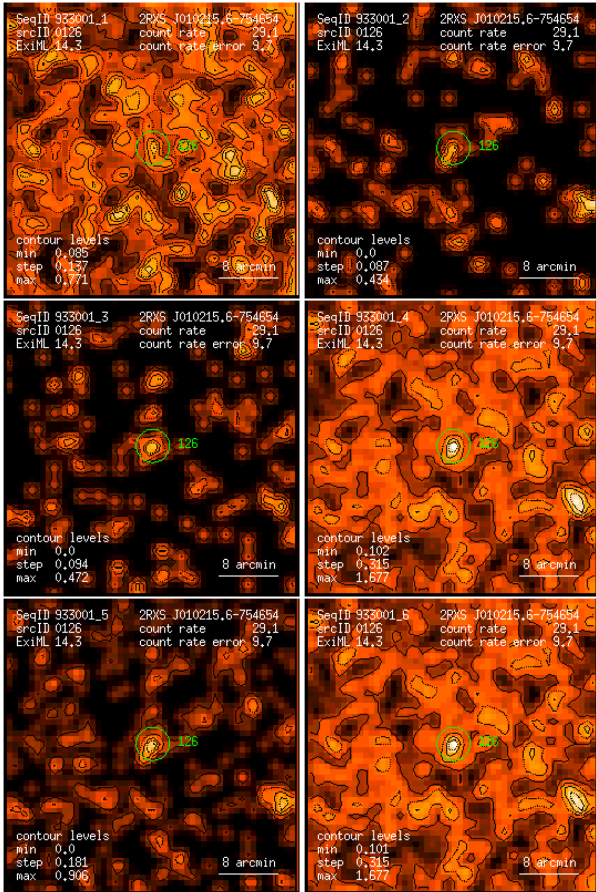
Figure 126: RASS 933001: detection 0126: band rate images, Gaussian filter: (1) PSPC channels 11 – 41, (2) 52 – 90, (3) 91 – 201, (4) 11 – 235, (5) 52 – 201, (6) 11 – 201. Broad band rates in counts/ks. Band rate contour levels in counts/ks/arcmin 2 .
