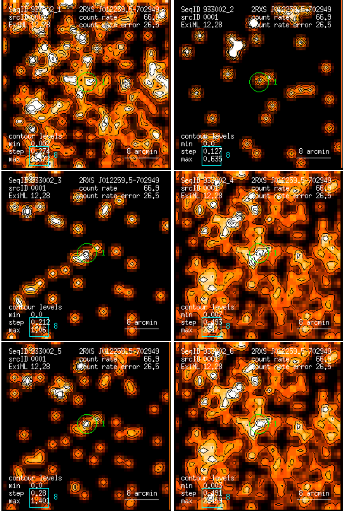
Figure 1: RASS 933002: detection 0001: band rate images, Gaussian filter: (1) PSPC channels 11 – 41, (2) 52 – 90, (3) 91 – 201, (4) 11 – 235, (5) 52 – 201, (6) 11 – 201. Broad band rates in counts/ks. Band rate contour levels in counts/ks/arcmin 2 .
