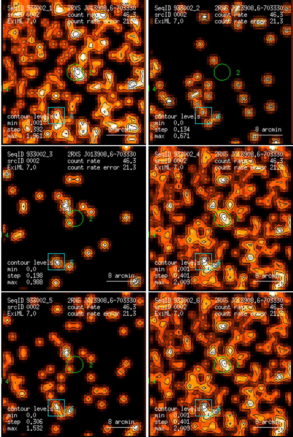
Figure 2: RASS 933002: detection 0002: band rate images, Gaussian filter: (1) PSPC channels 11 – 41, (2) 52 – 90, (3) 91 – 201, (4) 11 – 235, (5) 52 – 201, (6) 11 – 201. Broad band rates in counts/ks. Band rate contour levels in counts/ks/arcmin 2 .
