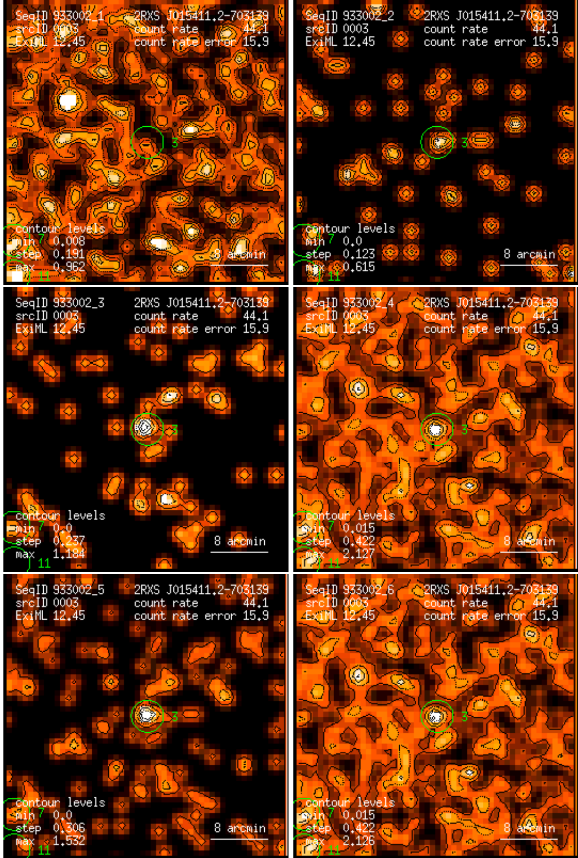
Figure 3: RASS 933002: detection 0003: band rate images, Gaussian filter: (1) PSPC channels 11 – 41, (2) 52 – 90, (3) 91 – 201, (4) 11 – 235, (5) 52 – 201, (6) 11 – 201. Broad band rates in counts/ks. Band rate contour levels in counts/ks/arcmin 2 .
