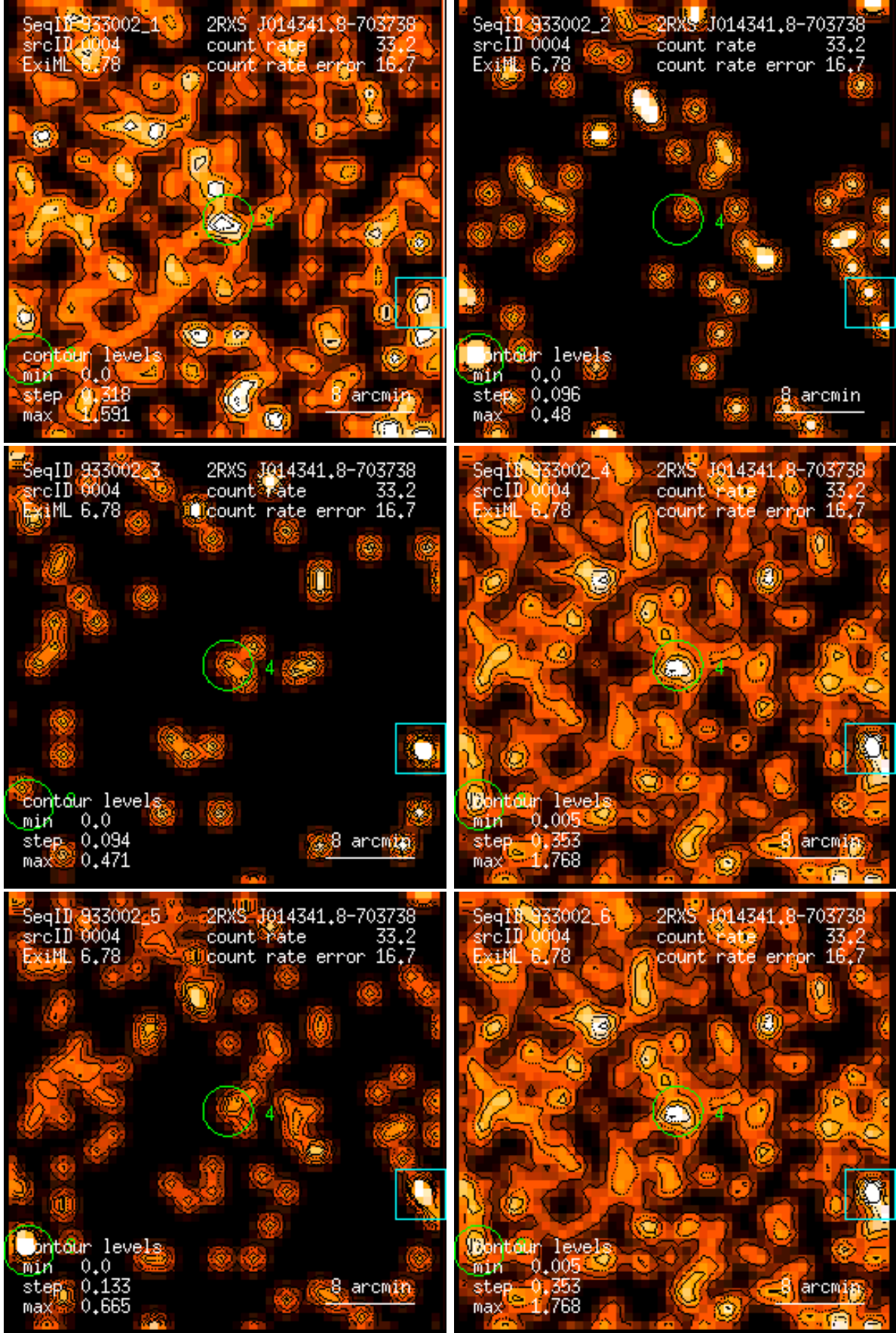
Figure 4: RASS 933002: detection 0004: band rate images, Gaussian filter: (1) PSPC channels 11 – 41, (2) 52 – 90, (3) 91 – 201, (4) 11 – 235, (5) 52 – 201, (6) 11 – 201. Broad band rates in counts/ks. Band rate contour levels in counts/ks/arcmin 2 .
