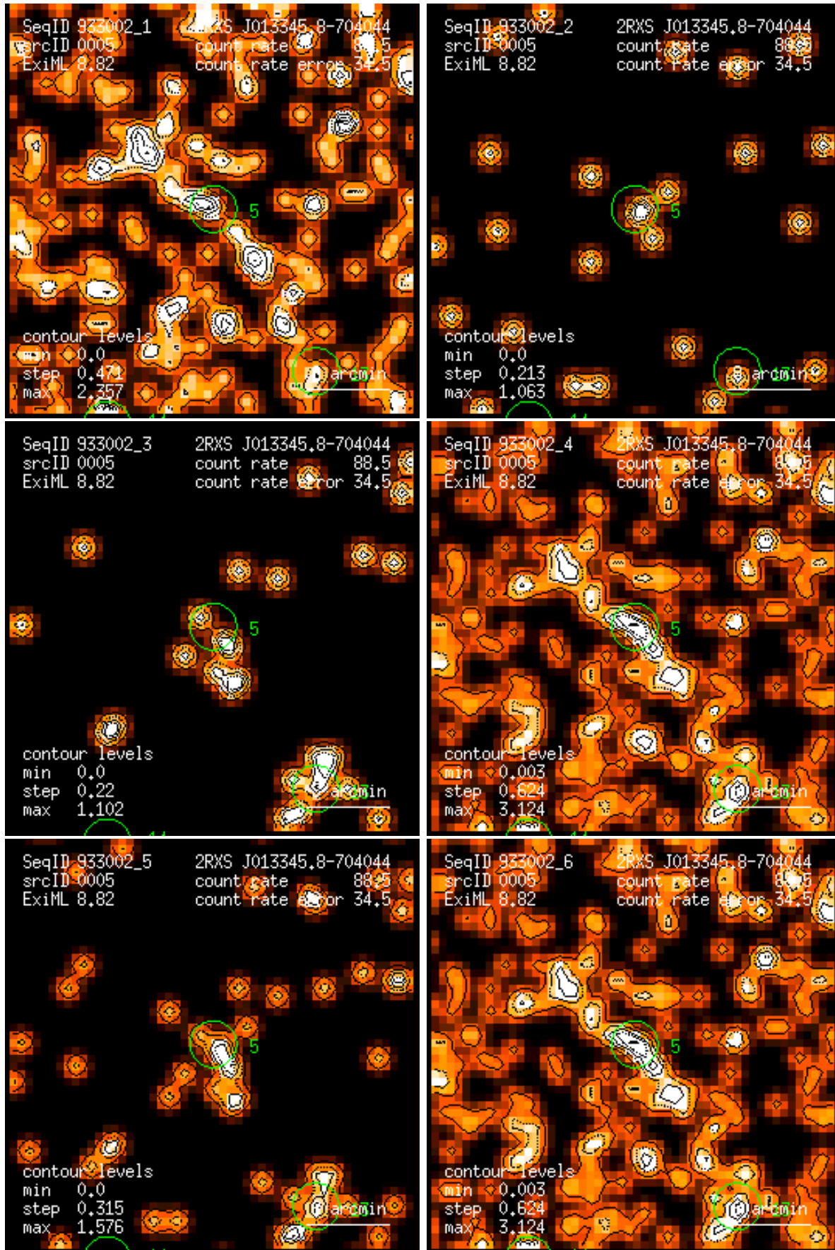
Figure 5: RASS 933002: detection 0005: band rate images, Gaussian filter: (1) PSPC channels 11 – 41, (2) 52 – 90, (3) 91 – 201, (4) 11 – 235, (5) 52 – 201, (6) 11 – 201. Broad band rates in counts/ks. Band rate contour levels in counts/ks/arcmin 2 .
