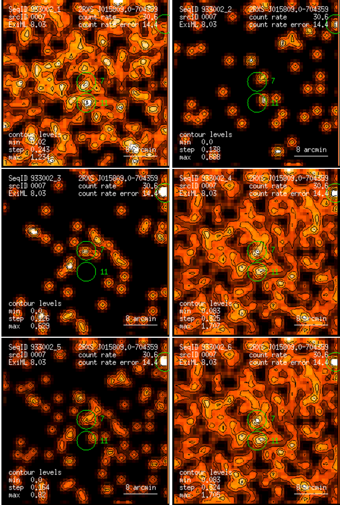
Figure 7: RASS 933002: detection 0007: band rate images, Gaussian filter: (1) PSPC channels 11 – 41, (2) 52 – 90, (3) 91 – 201, (4) 11 – 235, (5) 52 – 201, (6) 11 – 201. Broad band rates in counts/ks. Band rate contour levels in counts/ks/arcmin 2 .
