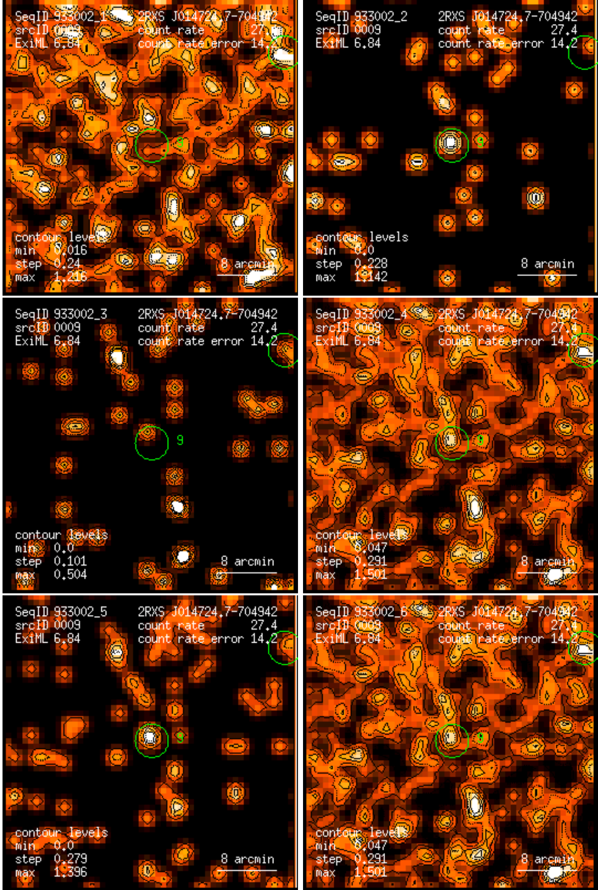
Figure 9: RASS 933002: detection 0009: band rate images, Gaussian filter: (1) PSPC channels 11 – 41, (2) 52 – 90, (3) 91 – 201, (4) 11 – 235, (5) 52 – 201, (6) 11 – 201. Broad band rates in counts/ks. Band rate contour levels in counts/ks/arcmin 2 .
