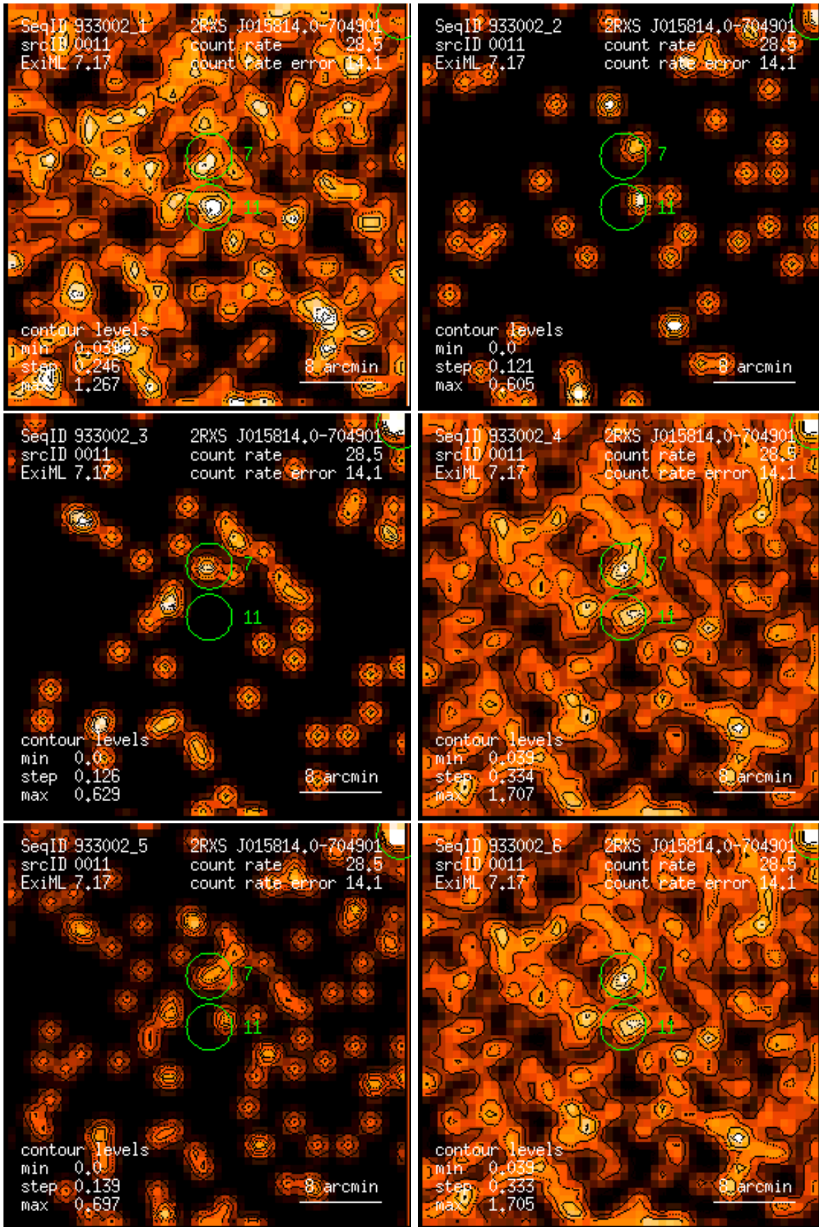
Figure 11: RASS 933002: detection 0011: band rate images, Gaussian filter: (1) PSPC channels 11 – 41, (2) 52 – 90, (3) 91 – 201, (4) 11 – 235, (5) 52 – 201, (6) 11 – 201. Broad band rates in counts/ks. Band rate contour levels in counts/ks/arcmin 2 .
