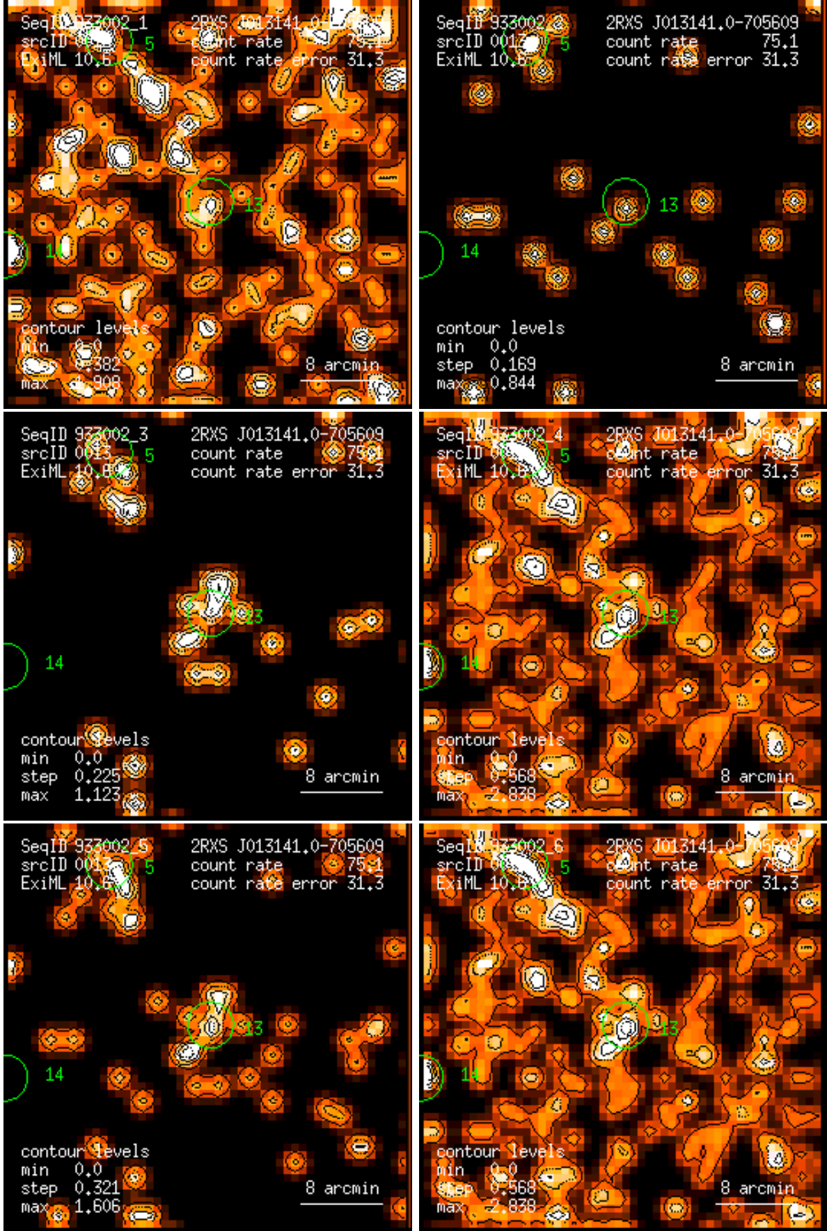
Figure 13: RASS 933002: detection 0013: band rate images, Gaussian filter: (1) PSPC channels 11 – 41, (2) 52 – 90, (3) 91 – 201, (4) 11 – 235, (5) 52 – 201, (6) 11 – 201. Broad band rates in counts/ks. Band rate contour levels in counts/ks/arcmin 2 .
