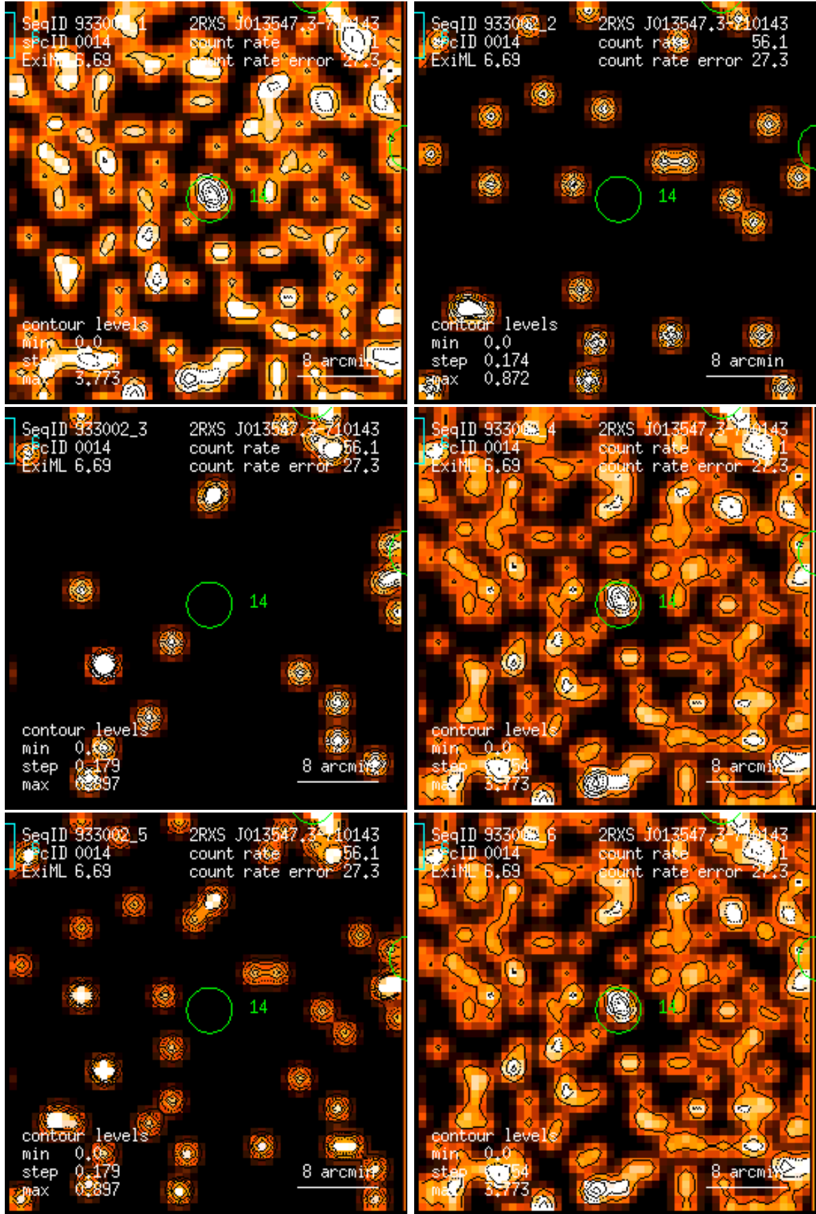
Figure 14: RASS 933002: detection 0014: band rate images, Gaussian filter: (1) PSPC channels 11 – 41, (2) 52 – 90, (3) 91 – 201, (4) 11 – 235, (5) 52 – 201, (6) 11 – 201. Broad band rates in counts/ks. Band rate contour levels in counts/ks/arcmin 2 .
