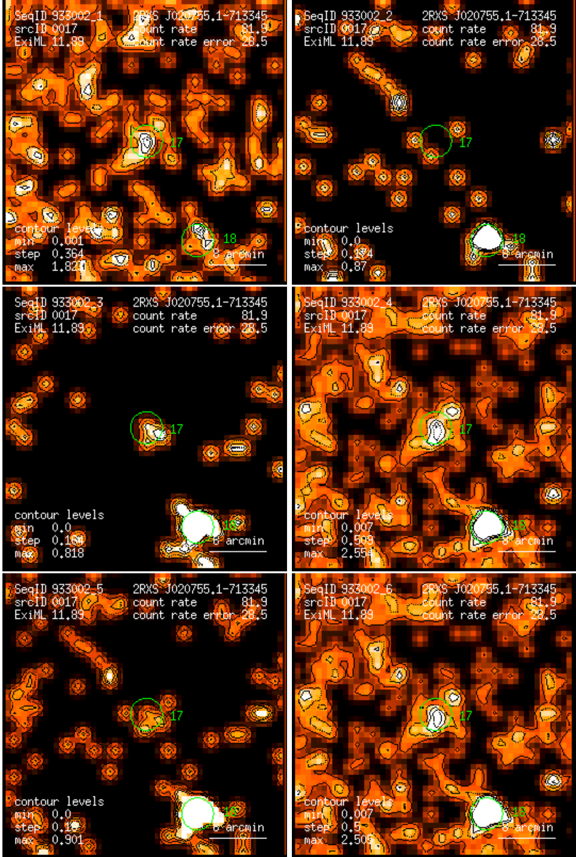
Figure 17: RASS 933002: detection 0017: band rate images, Gaussian filter: (1) PSPC channels 11 – 41, (2) 52 – 90, (3) 91 – 201, (4) 11 – 235, (5) 52 – 201, (6) 11 – 201. Broad band rates in counts/ks. Band rate contour levels in counts/ks/arcmin 2 .
