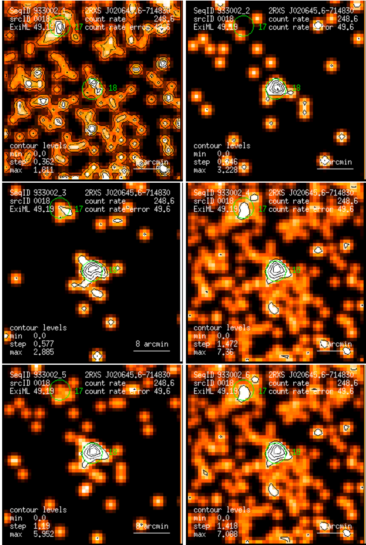
Figure 18: RASS 933002: detection 0018: band rate images, Gaussian filter: (1) PSPC channels 11 – 41, (2) 52 – 90, (3) 91 – 201, (4) 11 – 235, (5) 52 – 201, (6) 11 – 201. Broad band rates in counts/ks. Band rate contour levels in counts/ks/arcmin 2 .
