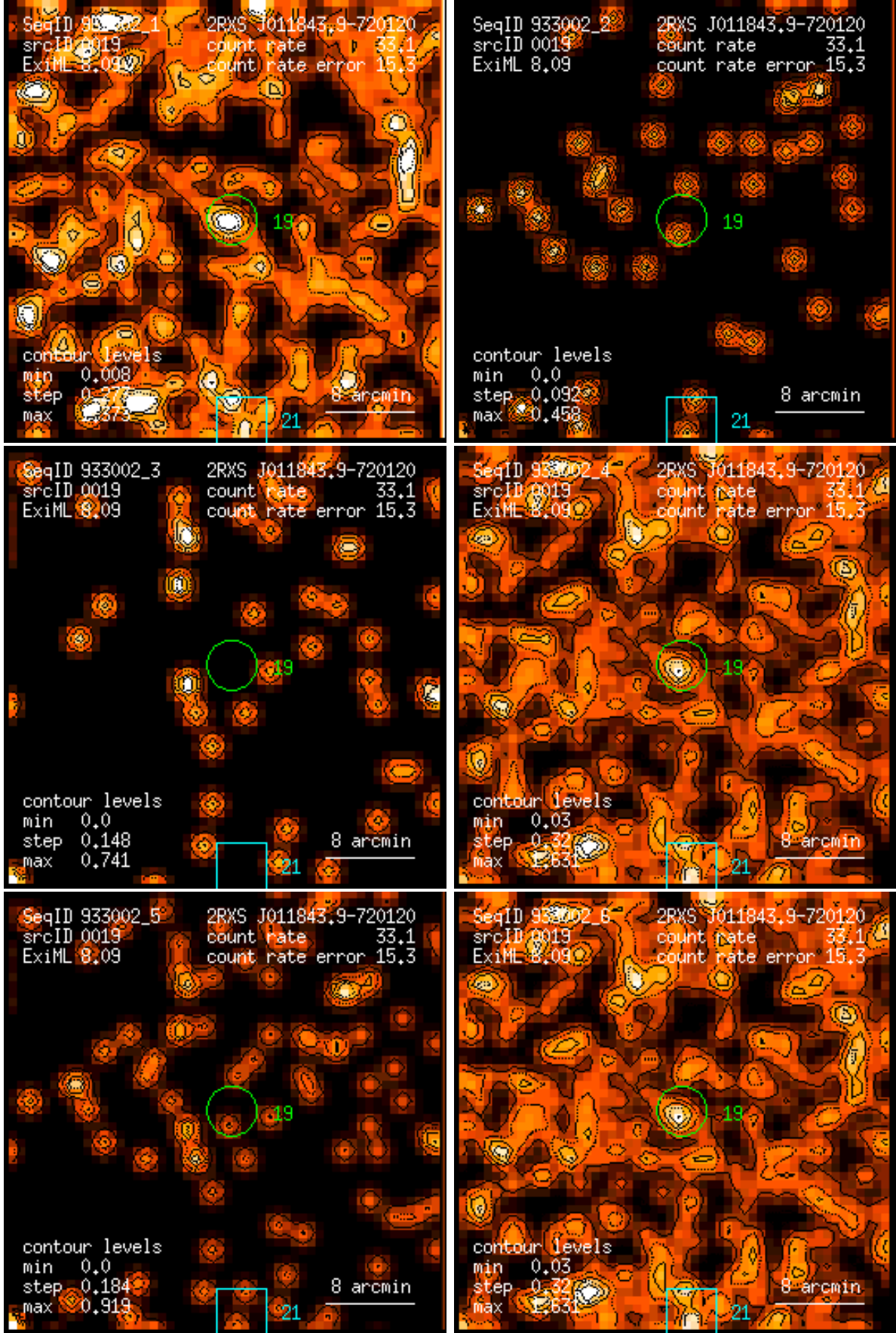
Figure 19: RASS 933002: detection 0019: band rate images, Gaussian filter: (1) PSPC channels 11 – 41, (2) 52 – 90, (3) 91 – 201, (4) 11 – 235, (5) 52 – 201, (6) 11 – 201. Broad band rates in counts/ks. Band rate contour levels in counts/ks/arcmin 2 .
