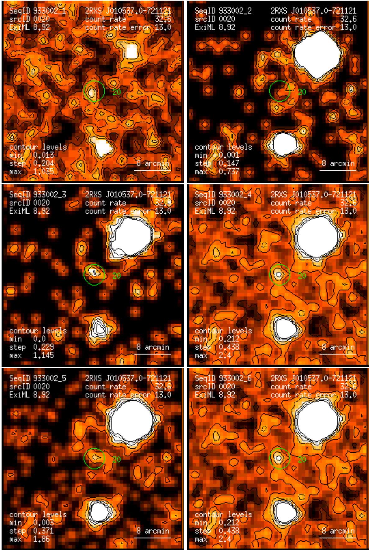
Figure 20: RASS 933002: detection 0020: band rate images, Gaussian filter: (1) PSPC channels 11 – 41, (2) 52 – 90, (3) 91 – 201, (4) 11 – 235, (5) 52 – 201, (6) 11 – 201. Broad band rates in counts/ks. Band rate contour levels in counts/ks/arcmin 2 .
