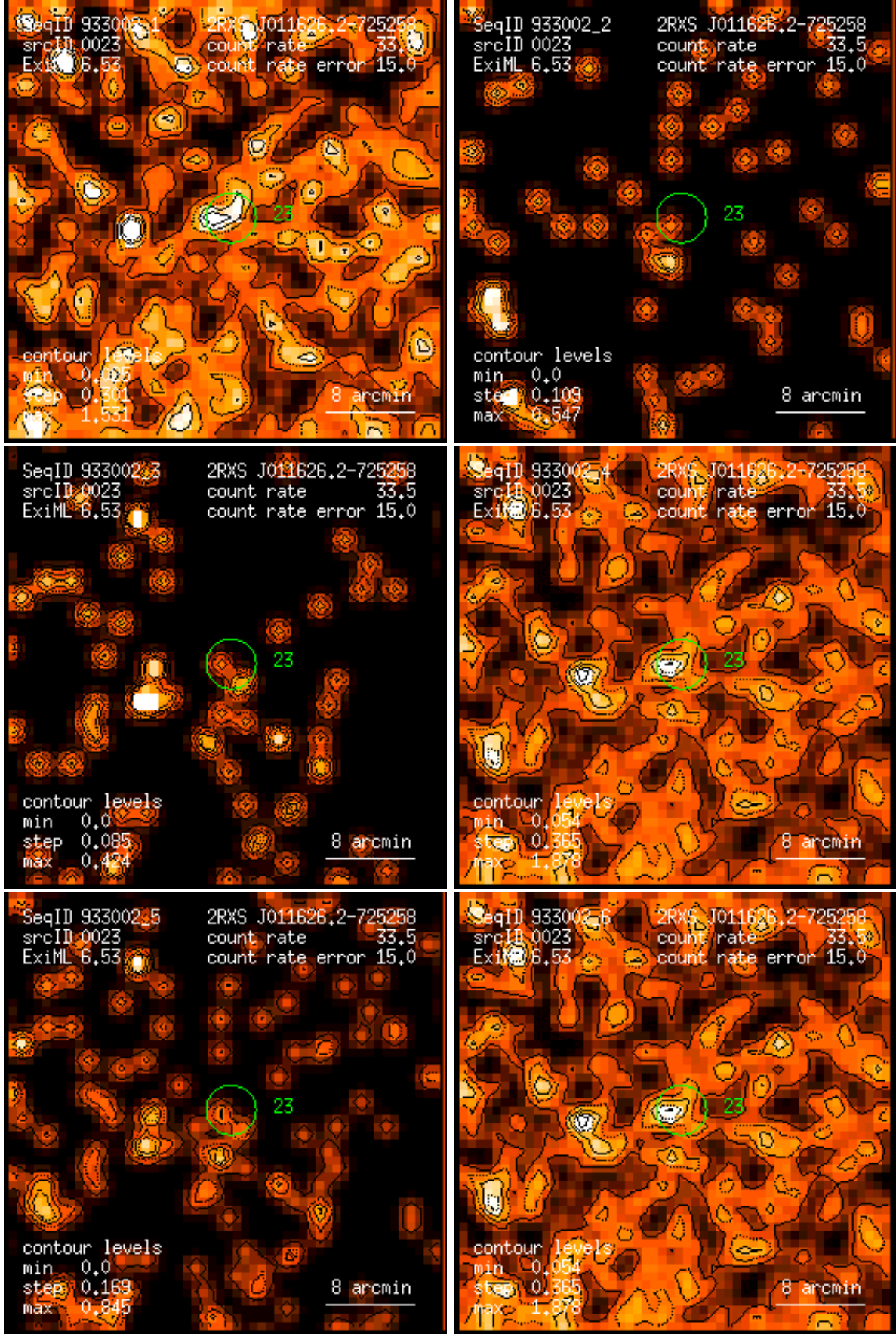
Figure 23: RASS 933002: detection 0023: band rate images, Gaussian filter: (1) PSPC channels 11 – 41, (2) 52 – 90, (3) 91 – 201, (4) 11 – 235, (5) 52 – 201, (6) 11 – 201. Broad band rates in counts/ks. Band rate contour levels in counts/ks/arcmin 2 .
