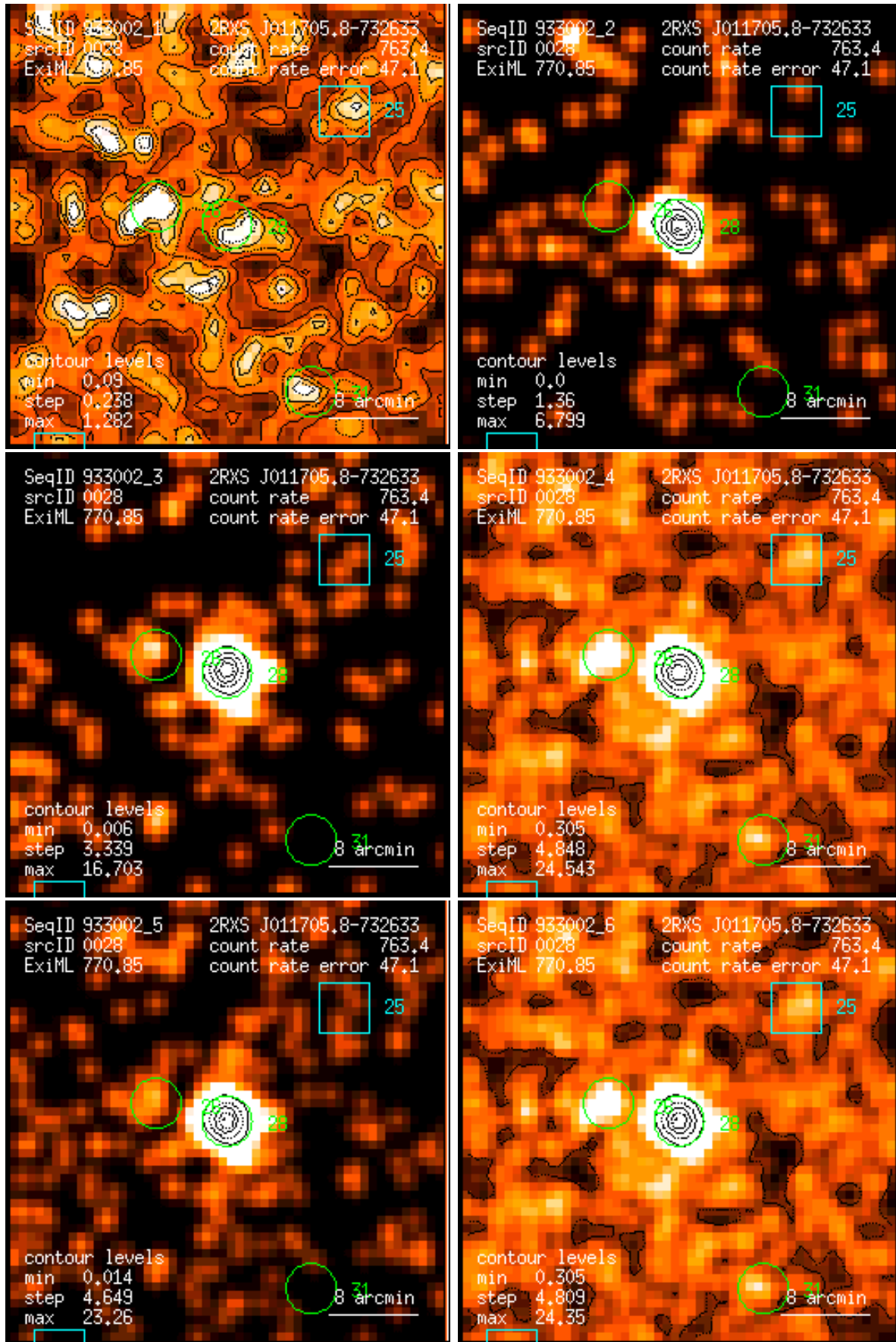
Figure 28: RASS 933002: detection 0028: band rate images, Gaussian filter: (1) PSPC channels 11 – 41, (2) 52 – 90, (3) 91 – 201, (4) 11 – 235, (5) 52 – 201, (6) 11 – 201. Broad band rates in counts/ks. Band rate contour levels in counts/ks/arcmin 2 .
