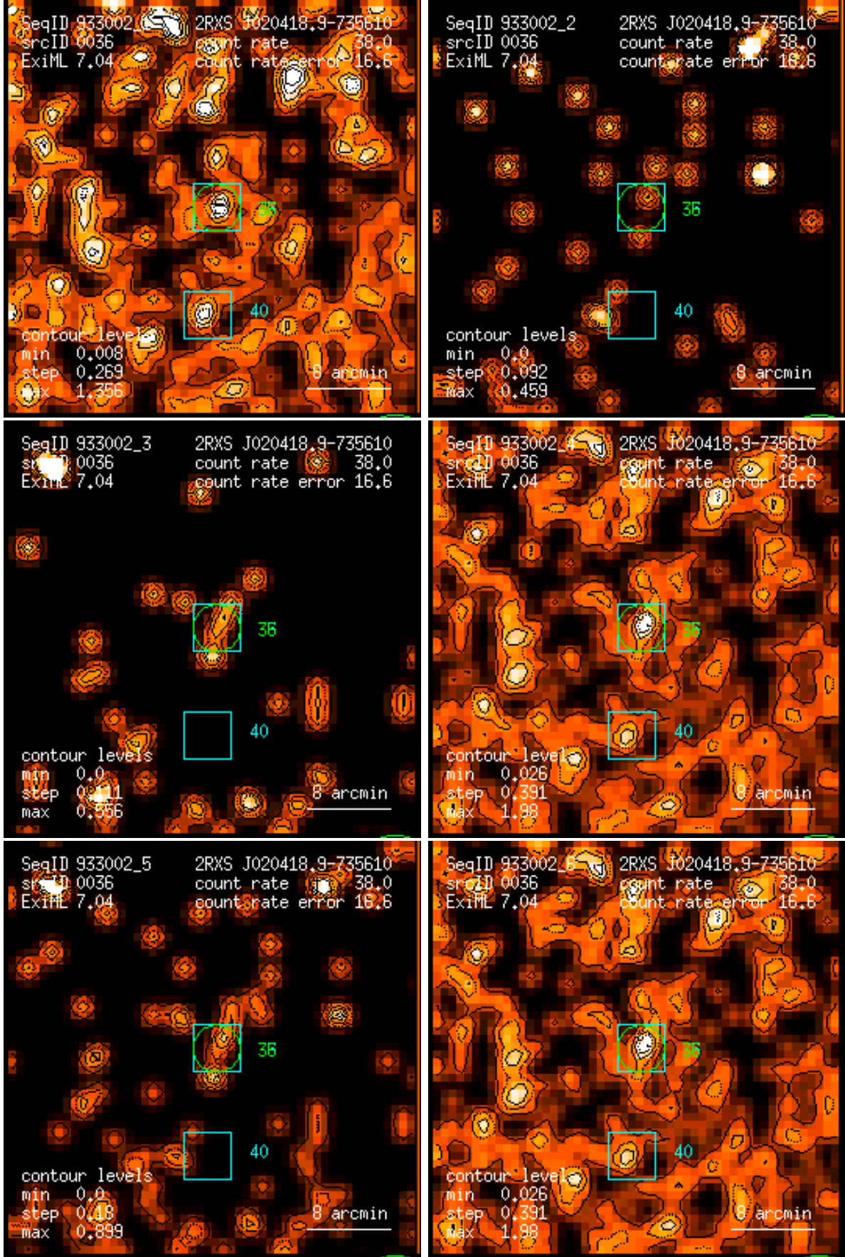
Figure 36: RASS 933002: detection 0036: band rate images, Gaussian filter: (1) PSPC channels 11 – 41, (2) 52 – 90, (3) 91 – 201, (4) 11 – 235, (5) 52 – 201, (6) 11 – 201. Broad band rates in counts/ks. Band rate contour levels in counts/ks/arcmin 2 .
