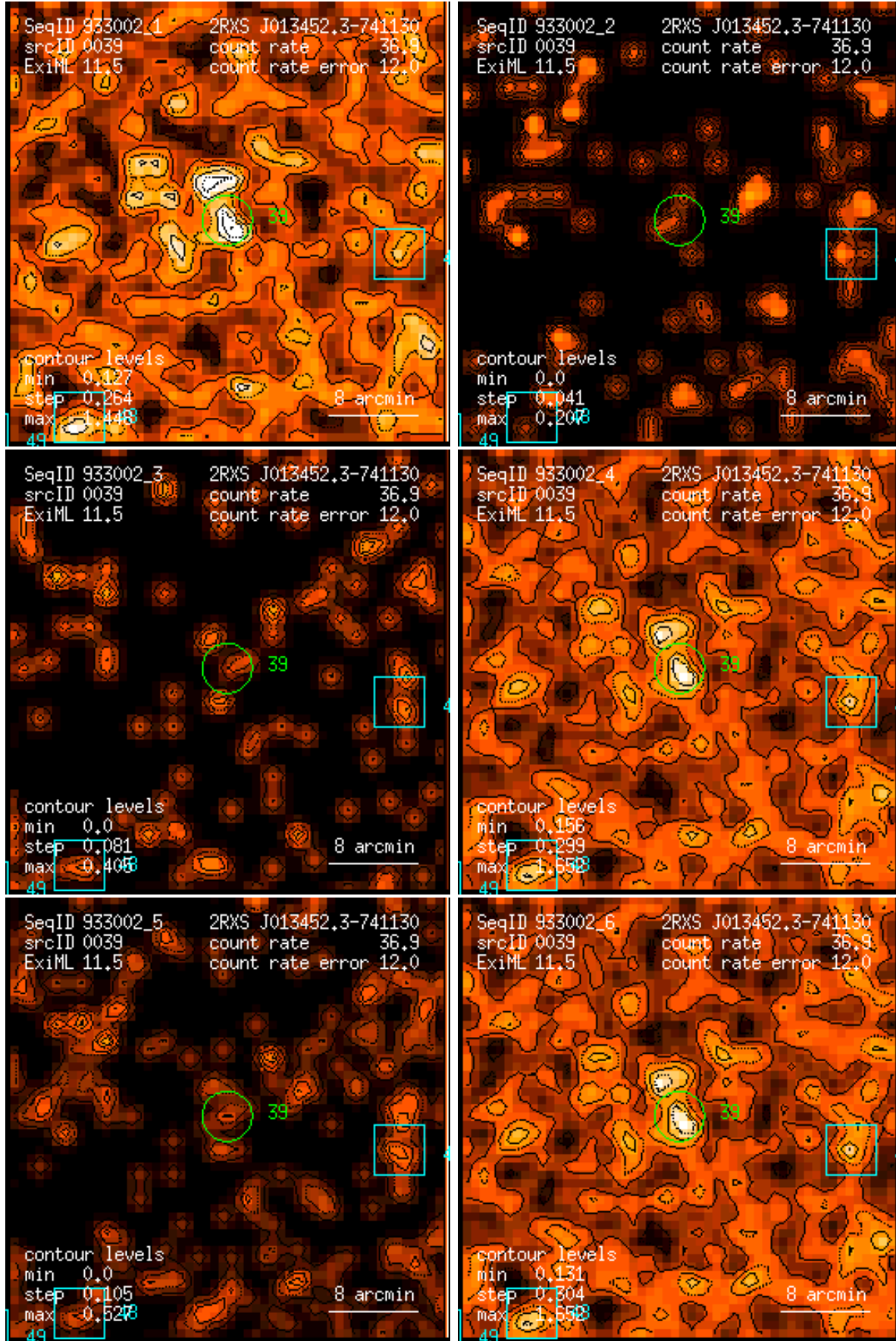
Figure 39: RASS 933002: detection 0039: band rate images, Gaussian filter: (1) PSPC channels 11 – 41, (2) 52 – 90, (3) 91 – 201, (4) 11 – 235, (5) 52 – 201, (6) 11 – 201. Broad band rates in counts/ks. Band rate contour levels in counts/ks/arcmin 2 .
