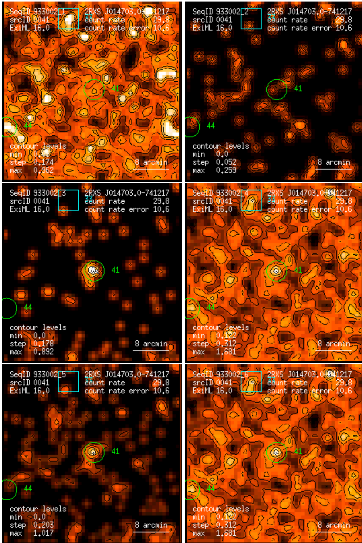
Figure 41: RASS 933002: detection 0041: band rate images, Gaussian filter: (1) PSPC channels 11 – 41, (2) 52 – 90, (3) 91 – 201, (4) 11 – 235, (5) 52 – 201, (6) 11 – 201. Broad band rates in counts/ks. Band rate contour levels in counts/ks/arcmin 2 .
