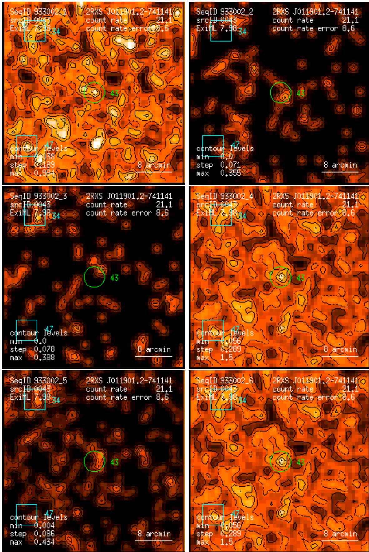
Figure 43: RASS 933002: detection 0043: band rate images, Gaussian filter: (1) PSPC channels 11 – 41, (2) 52 – 90, (3) 91 – 201, (4) 11 – 235, (5) 52 – 201, (6) 11 – 201. Broad band rates in counts/ks. Band rate contour levels in counts/ks/arcmin 2 .
