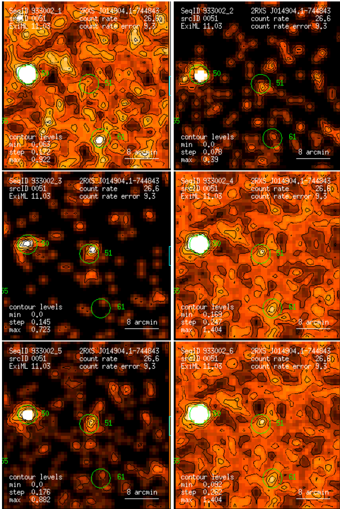
Figure 51: RASS 933002: detection 0051: band rate images, Gaussian filter: (1) PSPC channels 11 – 41, (2) 52 – 90, (3) 91 – 201, (4) 11 – 235, (5) 52 – 201, (6) 11 – 201. Broad band rates in counts/ks. Band rate contour levels in counts/ks/arcmin 2 .
