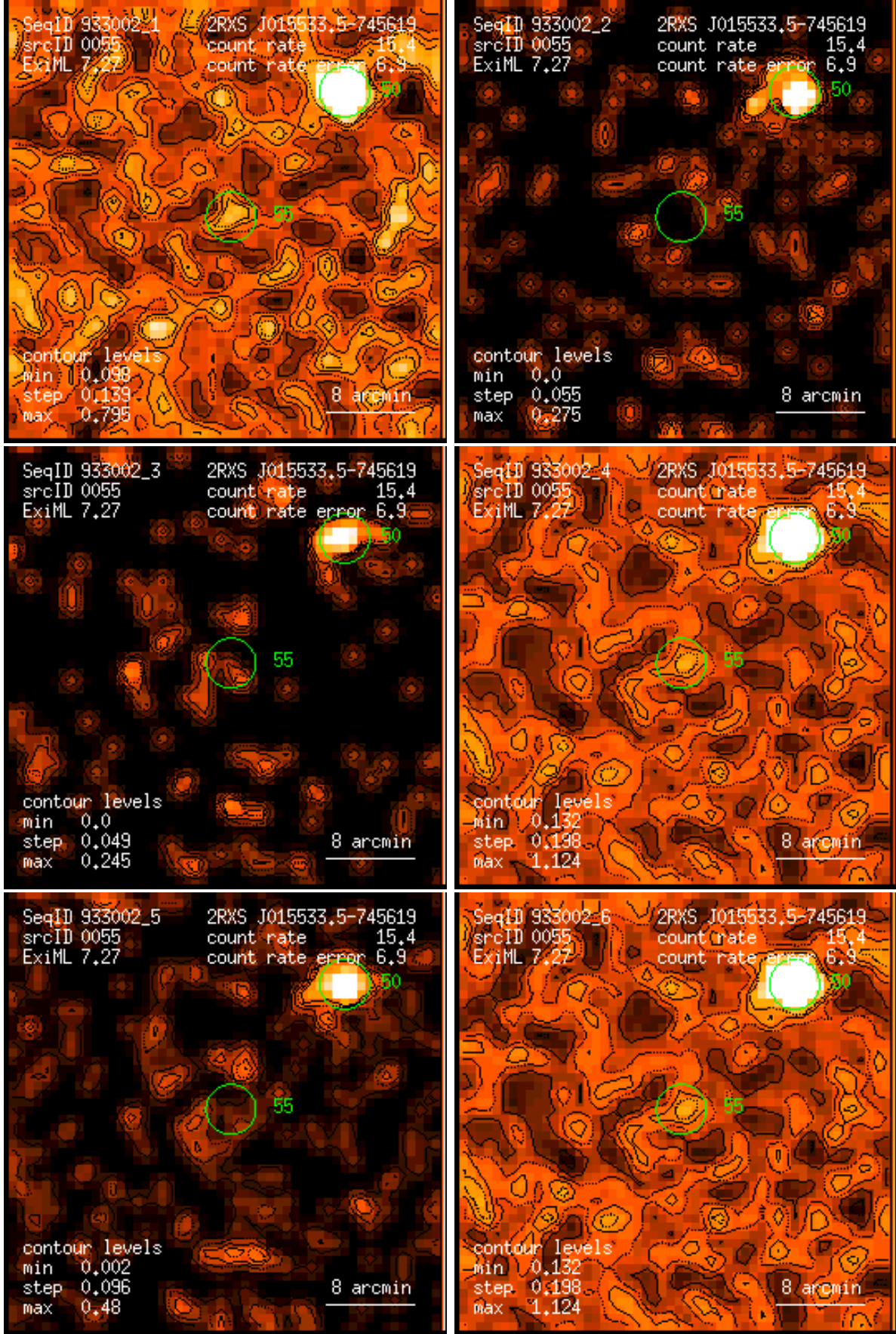
Figure 55: RASS 933002: detection 0055: band rate images, Gaussian filter: (1) PSPC channels 11 – 41, (2) 52 – 90, (3) 91 – 201, (4) 11 – 235, (5) 52 – 201, (6) 11 – 201. Broad band rates in counts/ks. Band rate contour levels in counts/ks/arcmin 2 .
