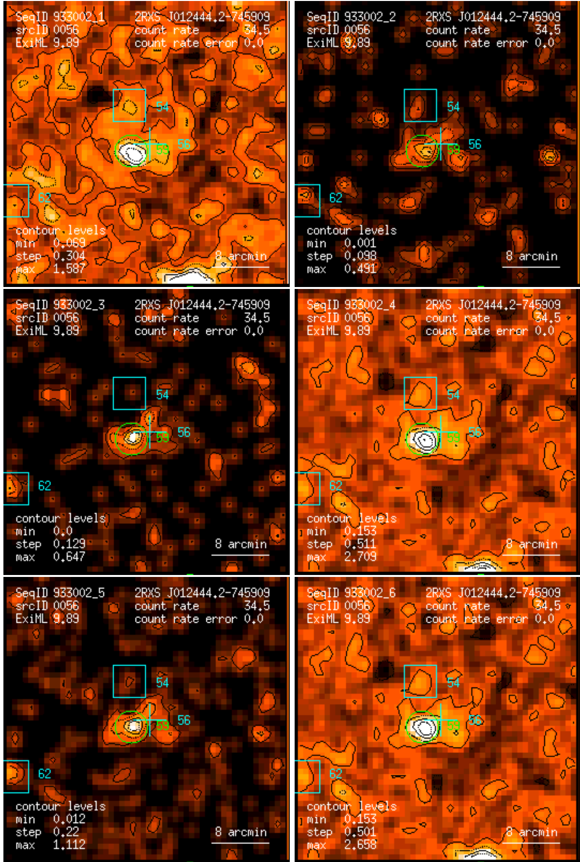
Figure 56: RASS 933002: detection 0056: band rate images, Gaussian filter: (1) PSPC channels 11 – 41, (2) 52 – 90, (3) 91 – 201, (4) 11 – 235, (5) 52 – 201, (6) 11 – 201. Broad band rates in counts/ks. Band rate contour levels in counts/ks/arcmin 2 .
