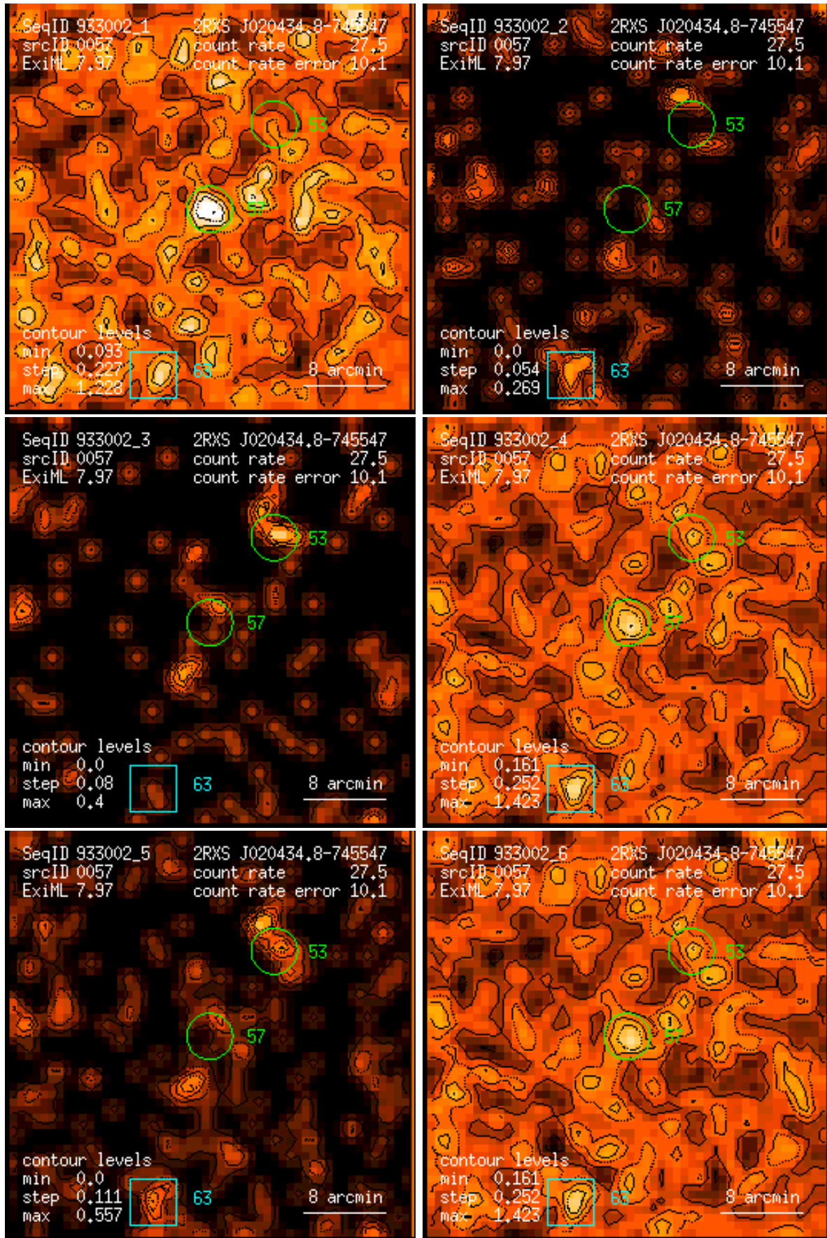
Figure 57: RASS 933002: detection 0057: band rate images, Gaussian filter: (1) PSPC channels 11 – 41, (2) 52 – 90, (3) 91 – 201, (4) 11 – 235, (5) 52 – 201, (6) 11 – 201. Broad band rates in counts/ks. Band rate contour levels in counts/ks/arcmin 2 .
